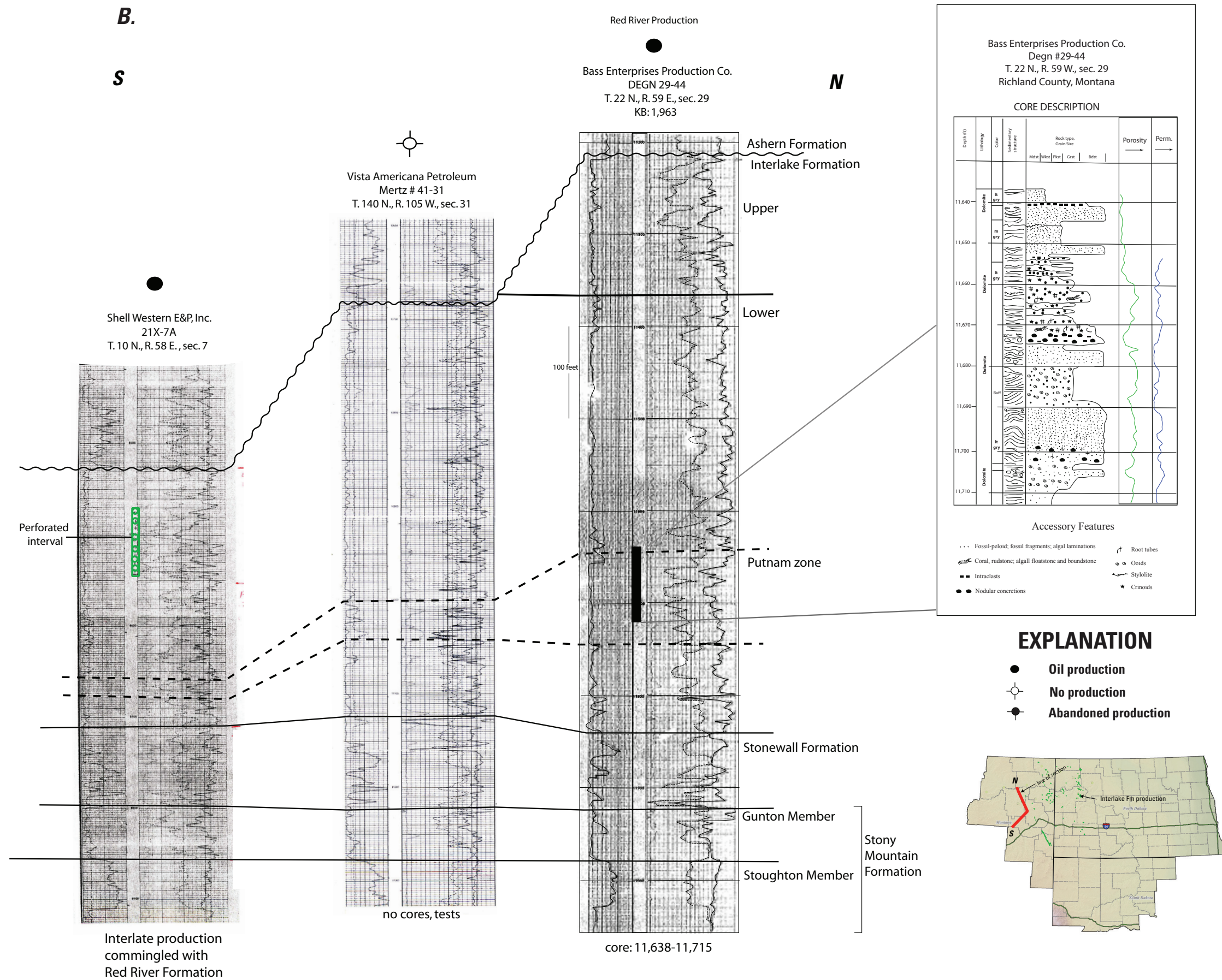
Figure 16. Wireline-log cross section showing formation contacts, producing intervals, and core description of the Interlake-Stonewall-Stony Mountain AU. Datum is on top of the Stoughton Member. Core description is modified from Inden and others (1988). oil; mcfg, thousand cubic feet of gas; bw, barrels of water; mbw, thousand barrels of water; DST, drill-stem test; KB, Kelly bushing elevation in feet; Mdst, mudstone; In core description, porosity column is green where porosity is greatest. (A) West-east section; (B) North-south section. BO, barrels of Wkst, wackestone; Pkst, packstone; Grst, grainstone; Bdst, boundstone.
