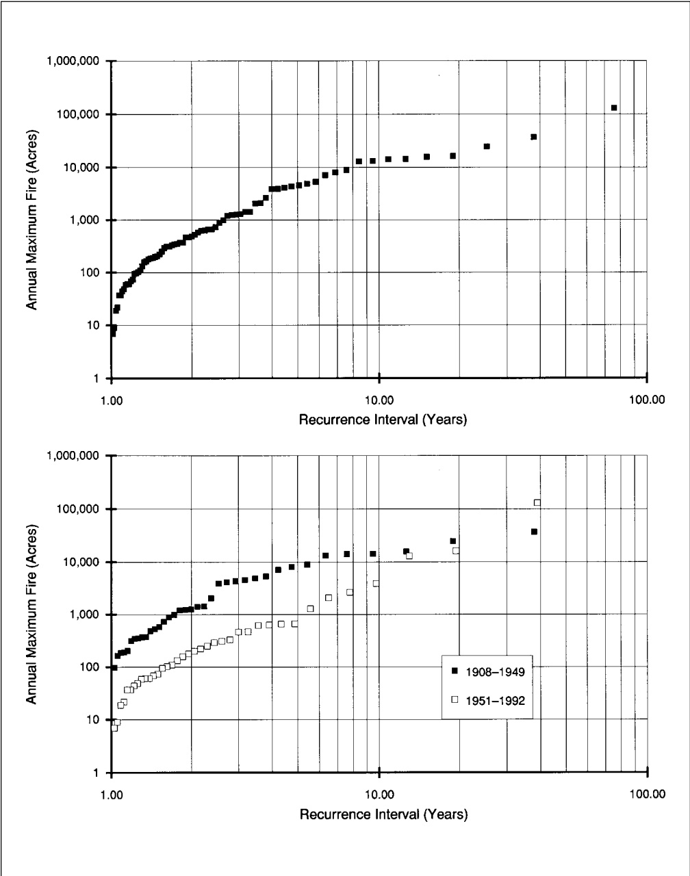
FIGURE 42.A4 Fire-frequency plots based on the annual maximum fire for all years of record (upper plot) and for the periods before and after 1950 (lower plot) for the Stanislaus National Forest.
