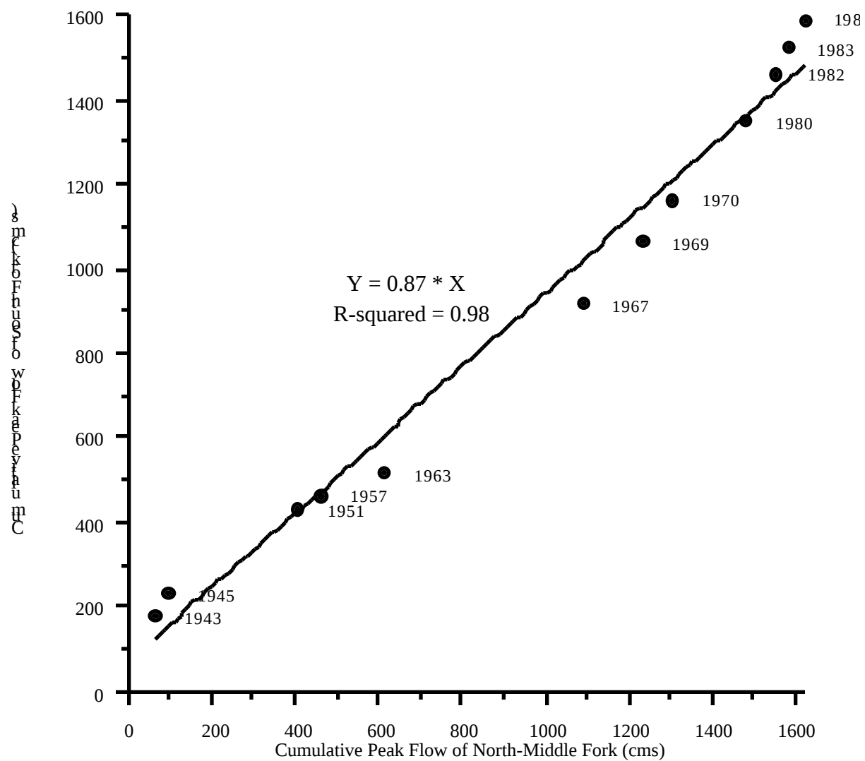
Figure 1. Double-mass plot of cumulative peak flows of the South Fork and North-Middle Fork Tule River. Curve was fitted by least-squares regression.
