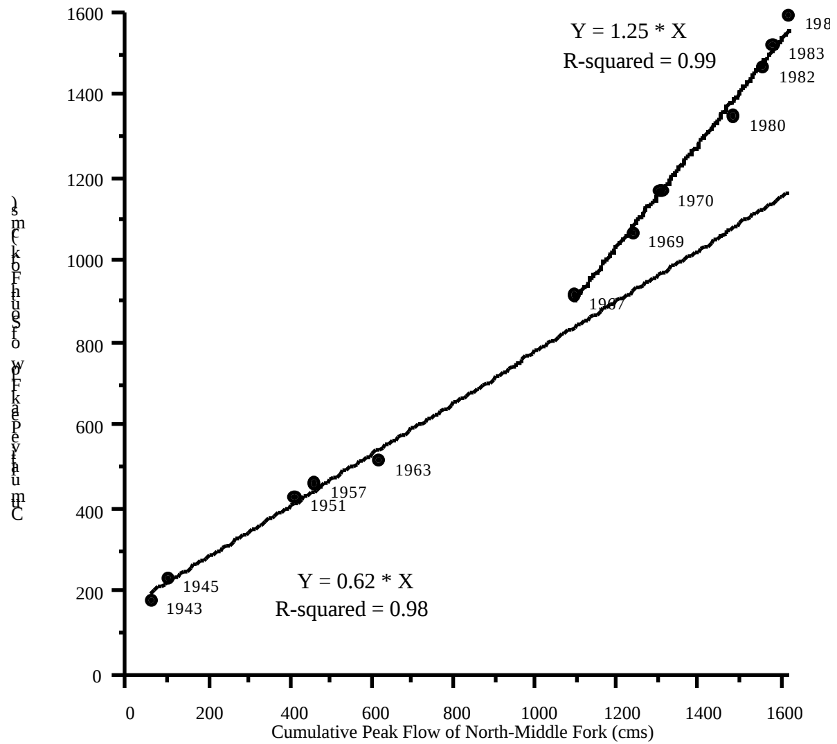
Figure 2. Double-mass plot of cumulative peak flows of the South Fork and North-Middle Fork Tule River for periods 1943-1963 and 1967-1984. Curves were fitted by least-squares regression.
