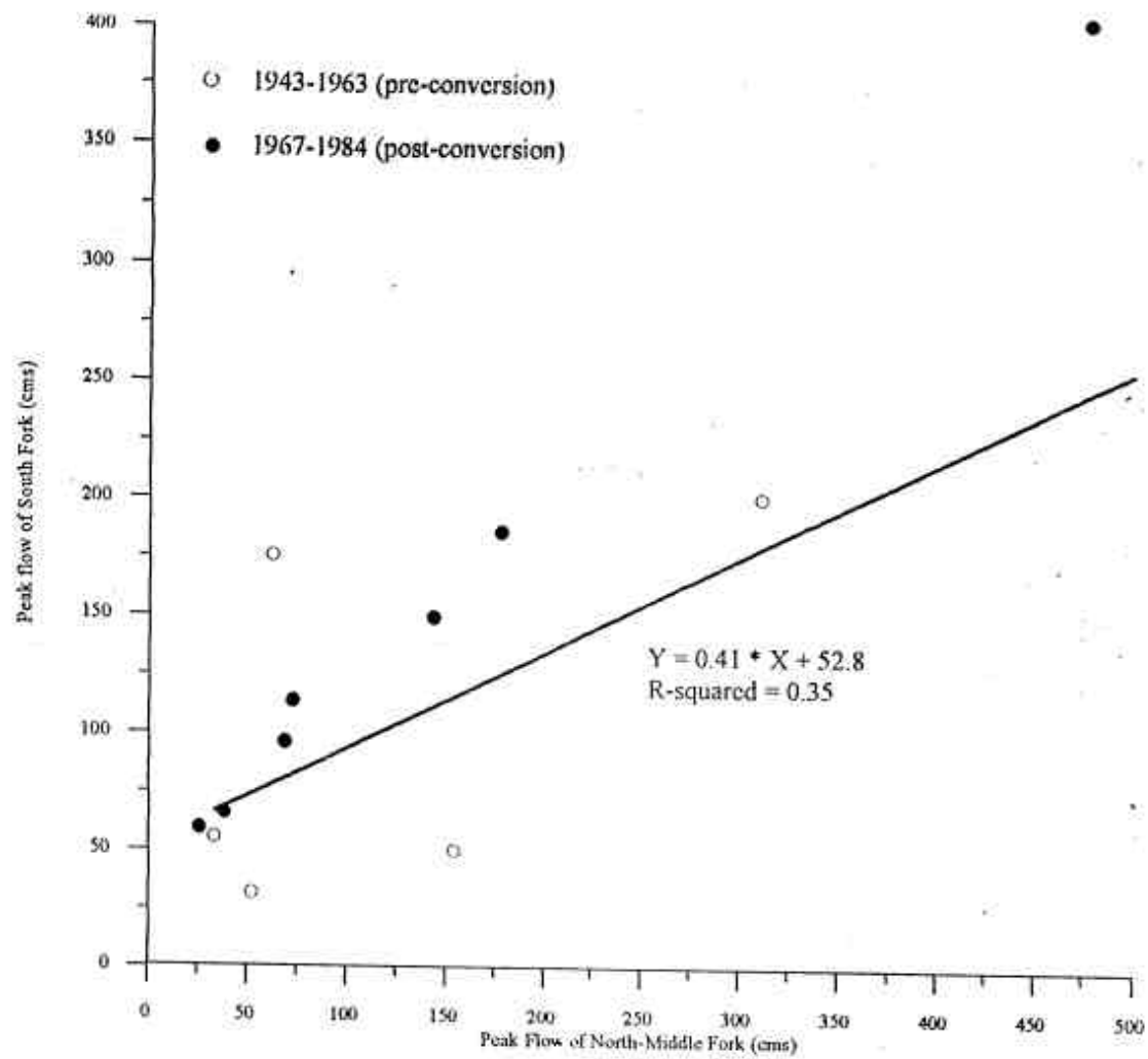
Figure 3. Relationship between annual peak flows on the South Fork and North-Middle Fork Tule River during the pre- and post-conversion periods. See text for explanation.
