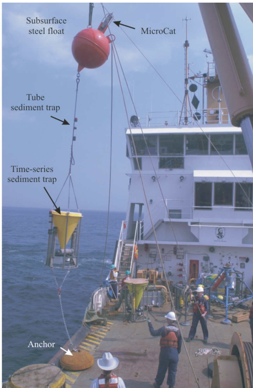
Figure 10. The subsurface mooring being deployed from the U.S. Coast Guard Cutter Marcus Hannah at Site B.
