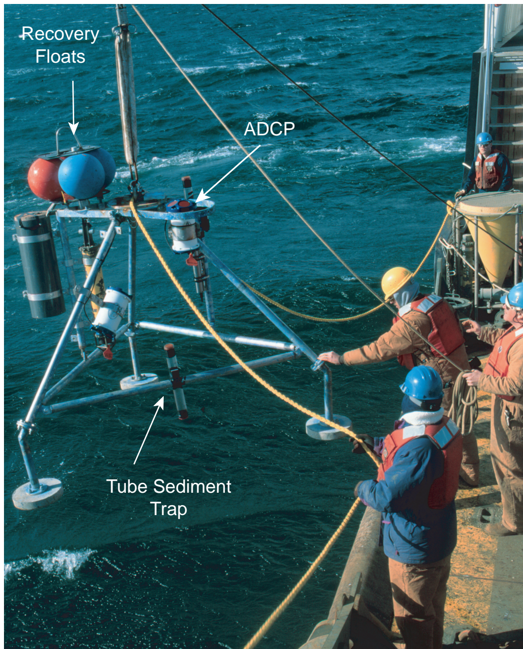
Figure 13C. Photograph of a small tripod frame used to deploy instrumentation at Site B being deployed from the U.S. Coast Guard Cutter White Heath. An Acoustic Doppler Current Profiler (ADCP) and tube sediment trap are attached to the tripod. The floats on the top of the frame are released by an acoustic release and pull a recovery line to the surface.
