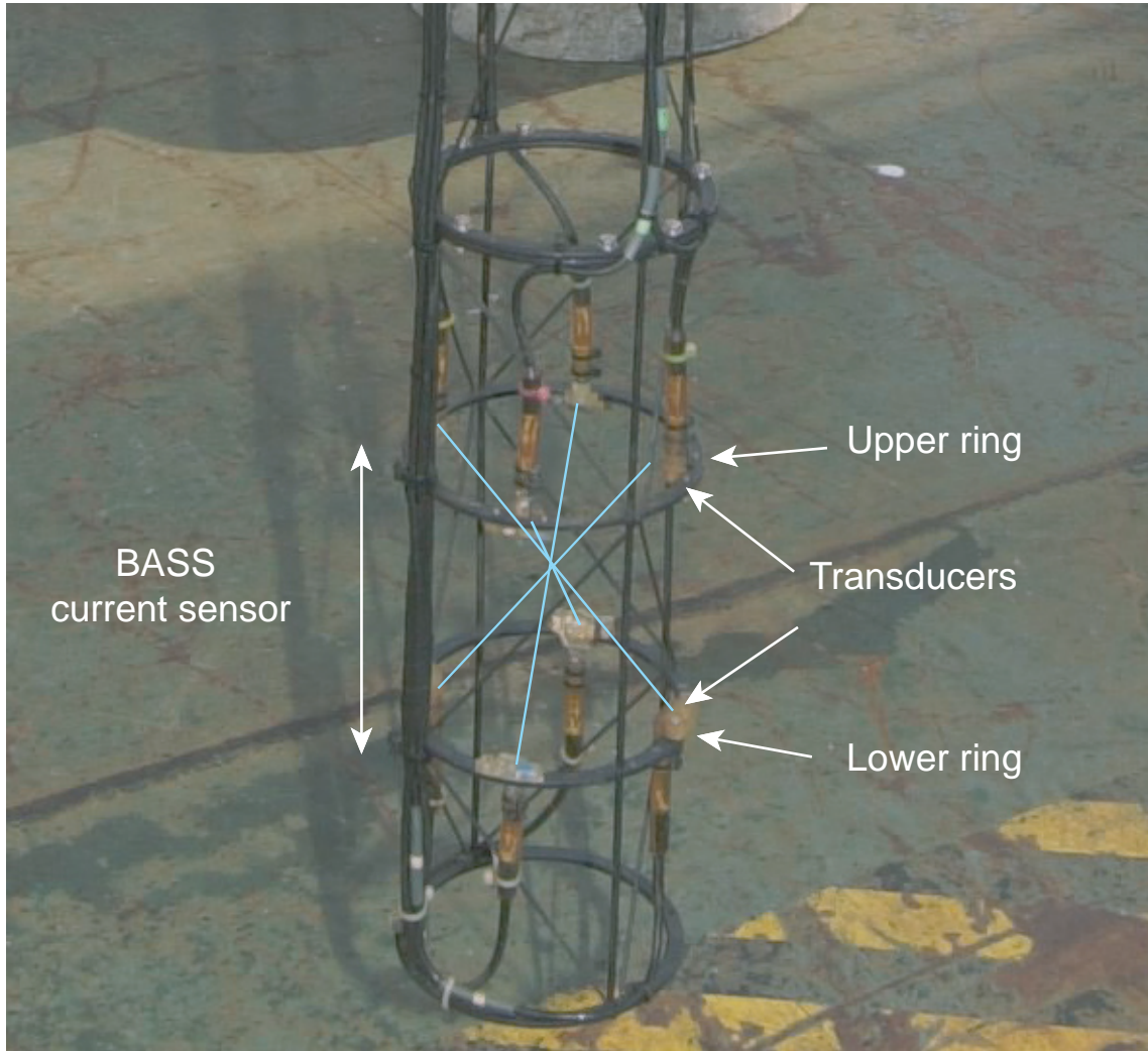
Figure 13E. Photograph of BASS current sensor. Currents are measured by pairs of acoustic sensors mounted on two rings spaced 20 cm apart vertically. The light blue lines indicate the acoustic paths between the four pairs of transducers on the upper and lower ring.
