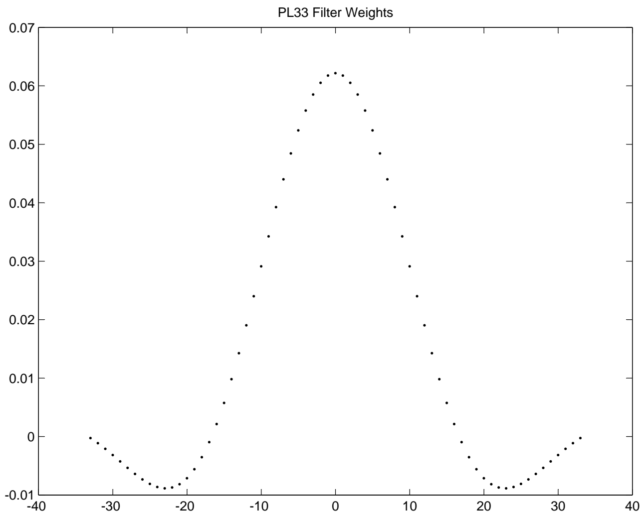
Figure 20: Filter weights applied to the time-series data in the low-pass filter PL33. The filter truncates 33 points from the beginning and end of each time series.
