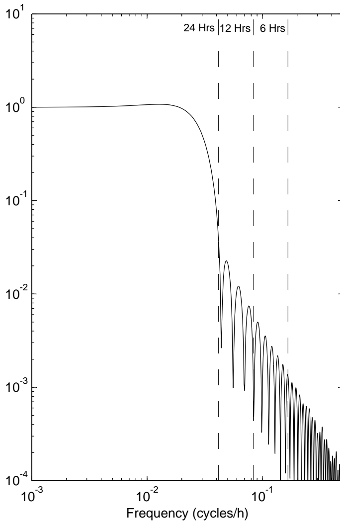
Figure 21: Amplitude transfer function for the low-pass filter PL33, showing the amplitude response as a function of frequency.
