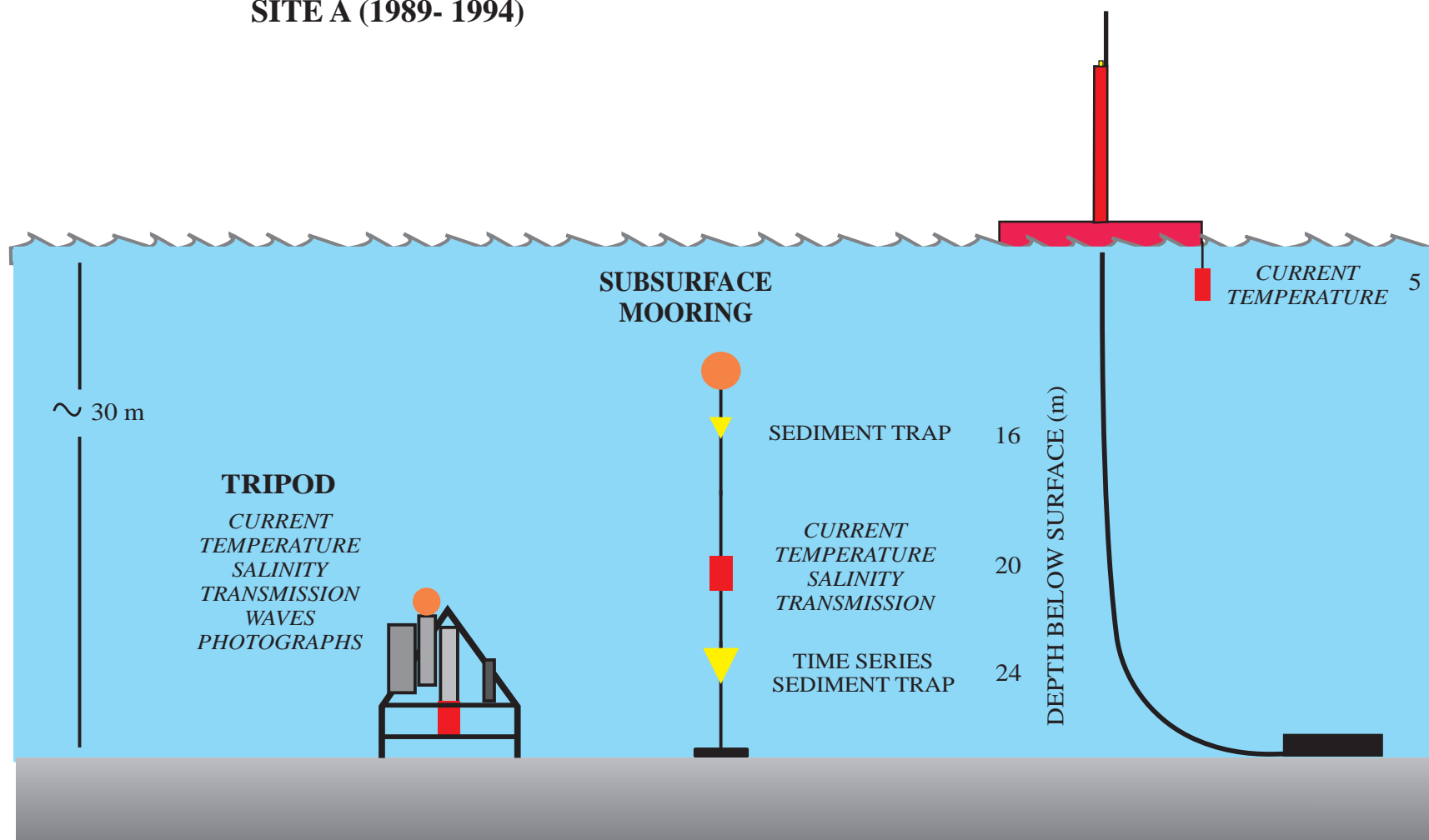
Figure 6A. Schematic of moored instruments at the long-term western Massachusetts Bay Site A (figure 1 and figure 4) from 1989 to 1994. During this period, instruments were deployed from the Large Navigational Buoy, on a subsurface mooring, and on a bottom tripod system. Nominal measurement depths are 1 m above bottom (mab), 10 mab, and 5 m below the surface.
