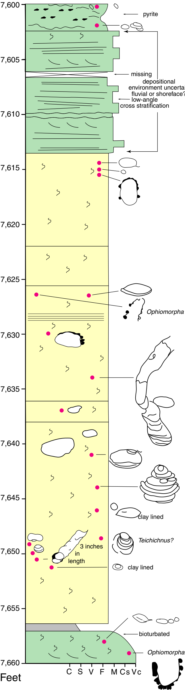
GRAPHIC LOG OF USGS CORE D122 OF THE FRONTIER FORMATION
