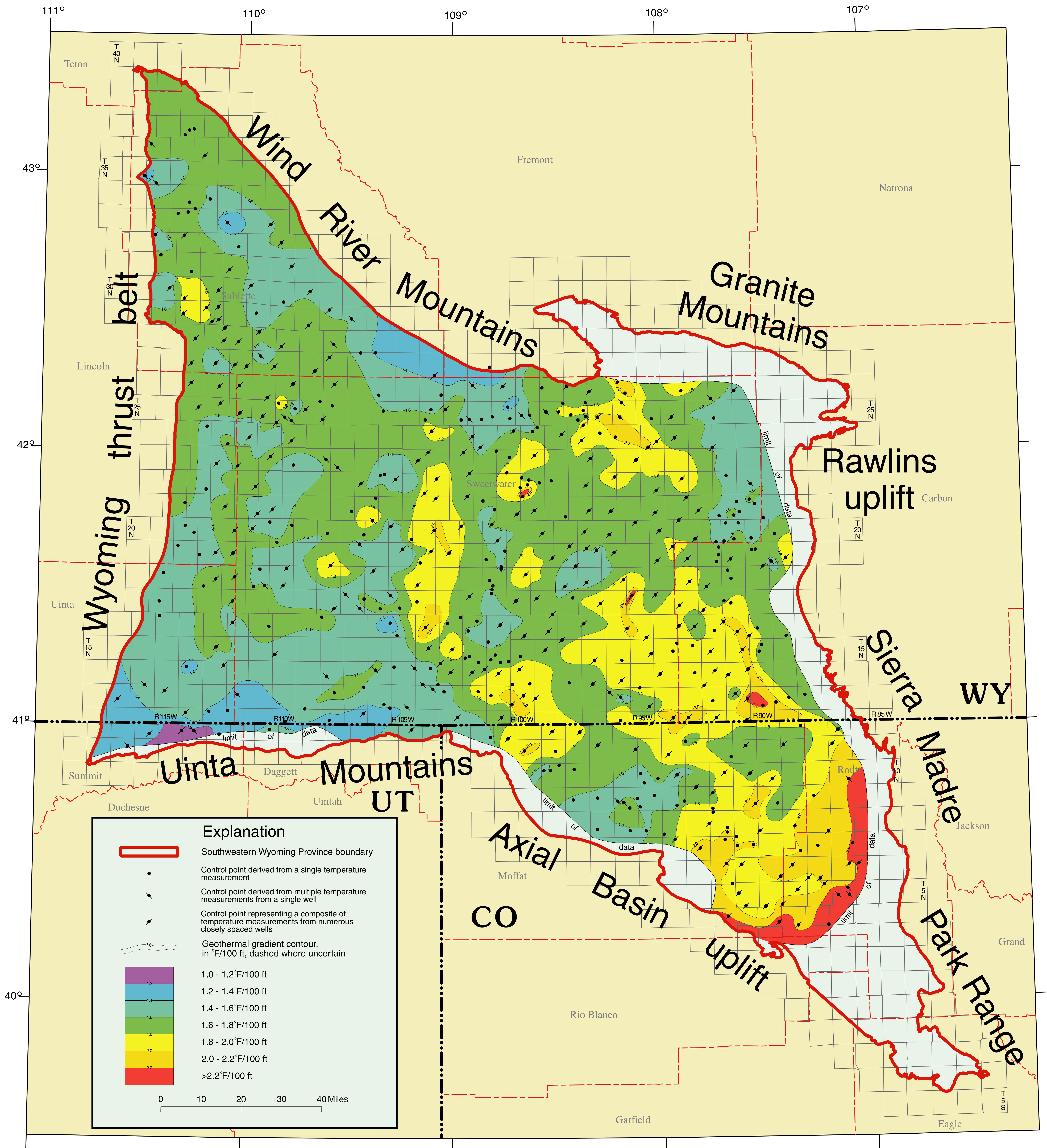
GEOHERMAL GRADIENT MAP OF THE SOUTHWESTERN WYOMING PROVINCE, SOUTHWESTERN WYOMING, NORTHWESTERN COLORADO, AND NORTHEASTERN UTAH
