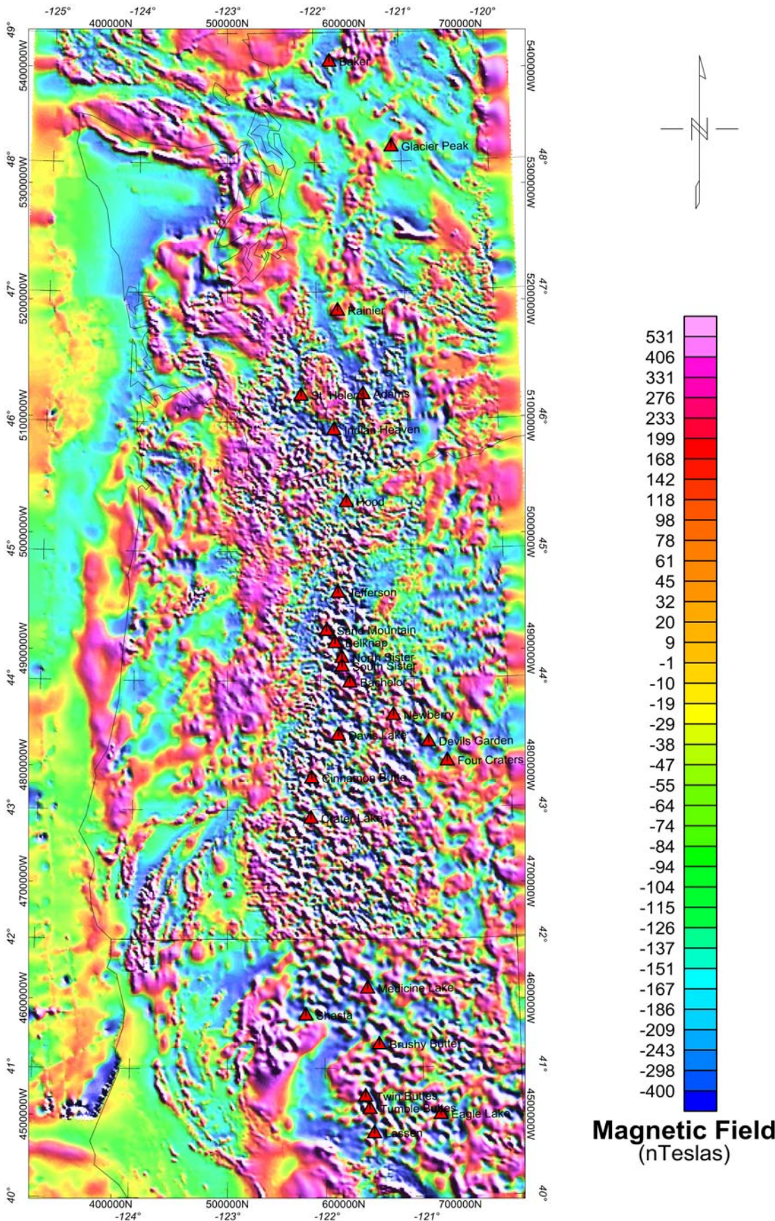
Magnetic Field Pacific Cascades Region
