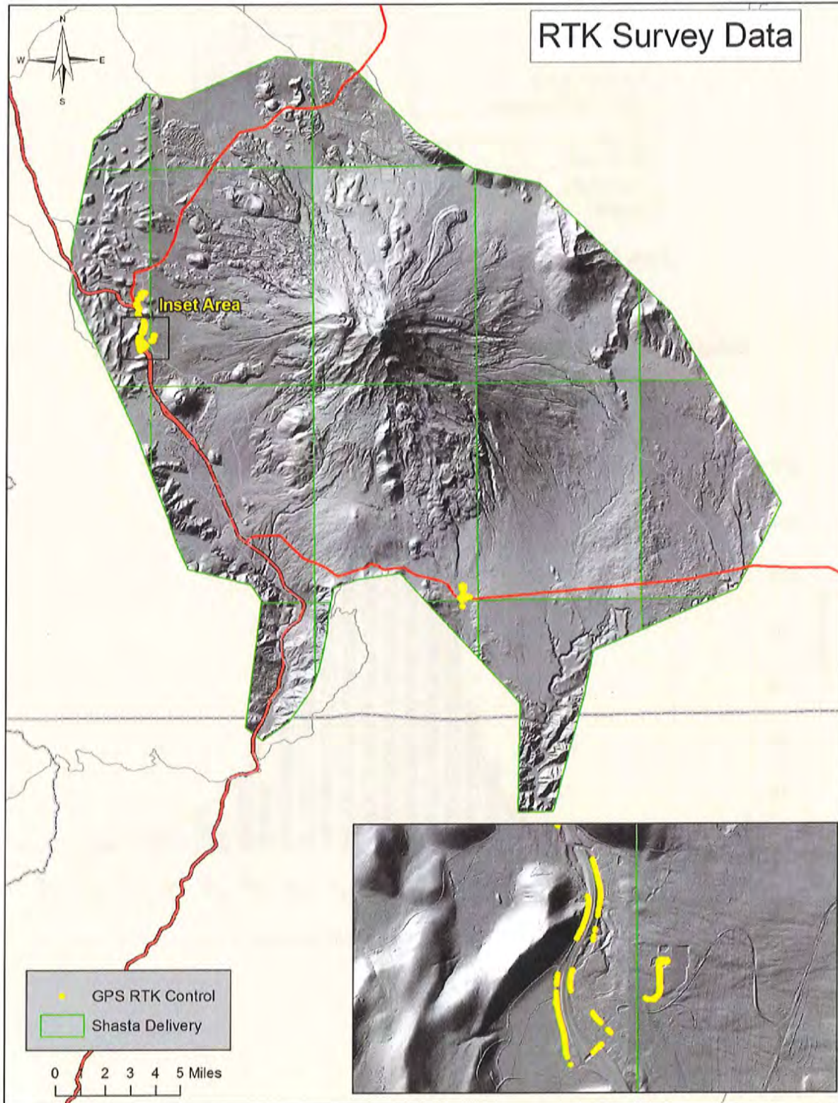
Figure 6. Locations of RTK control surveyed by DOGAMI. Data was used to test absolute accuracy for the Shasta CVO lidar survey within the Delivery extent.
