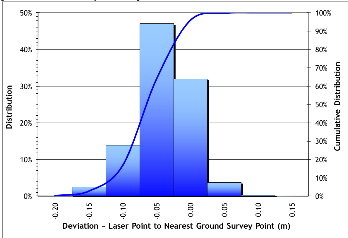
Figure 3.5. Mt. Shasta Study Area histogram statistics
