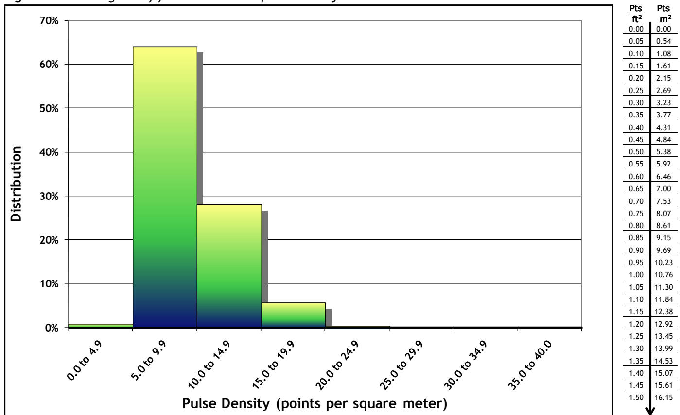
Figure 4.1. Histogram of first return laser pulse density.
