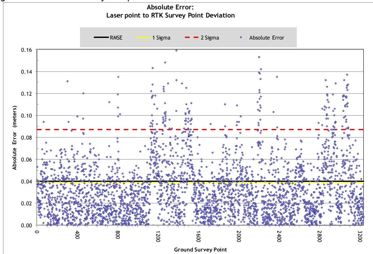
Figure 3.6. Mt. Shasta Study Area point absolute deviation statistics.
