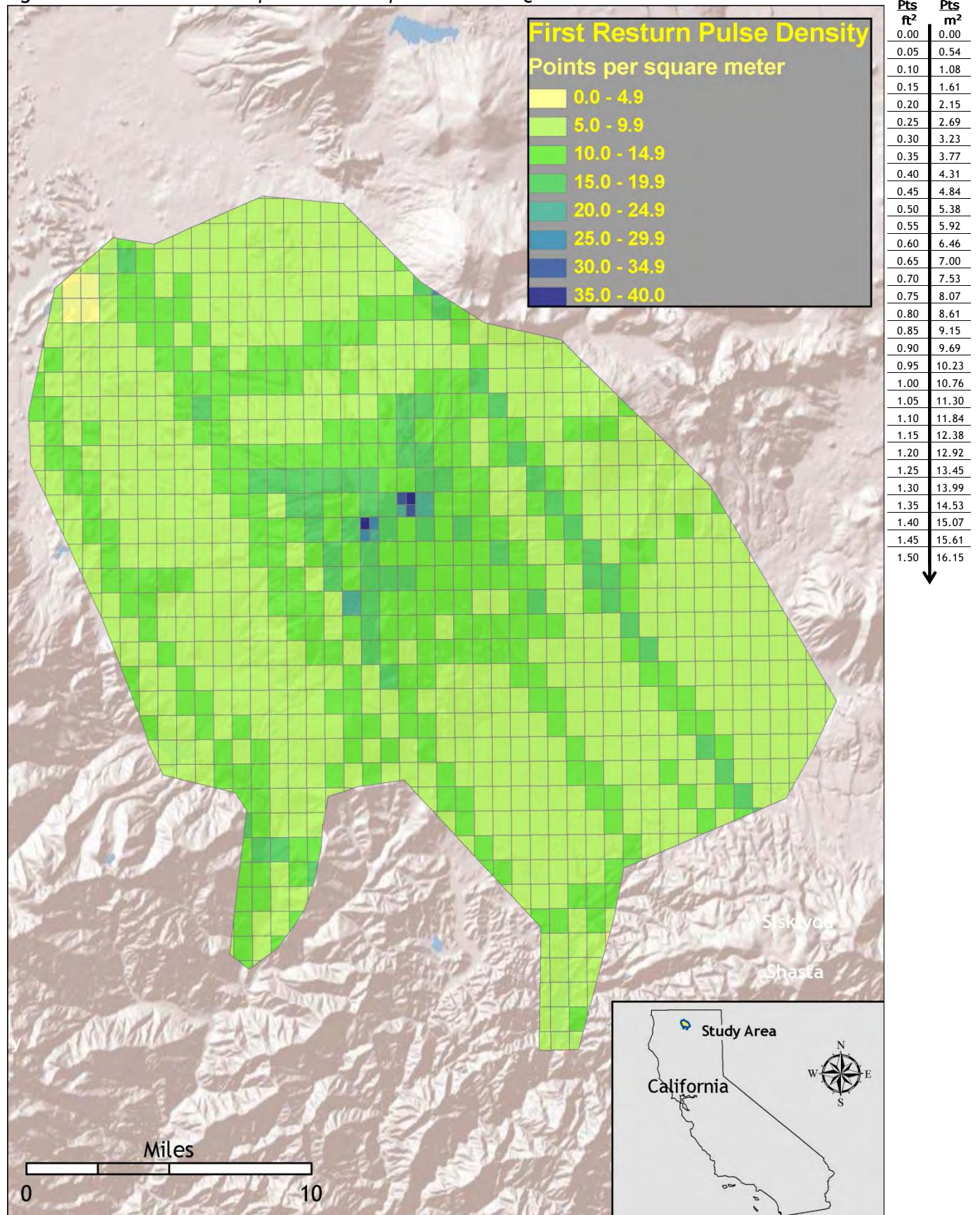
Figure 4.2. First return laser pulse densities per 0.75' USGS Quad.
