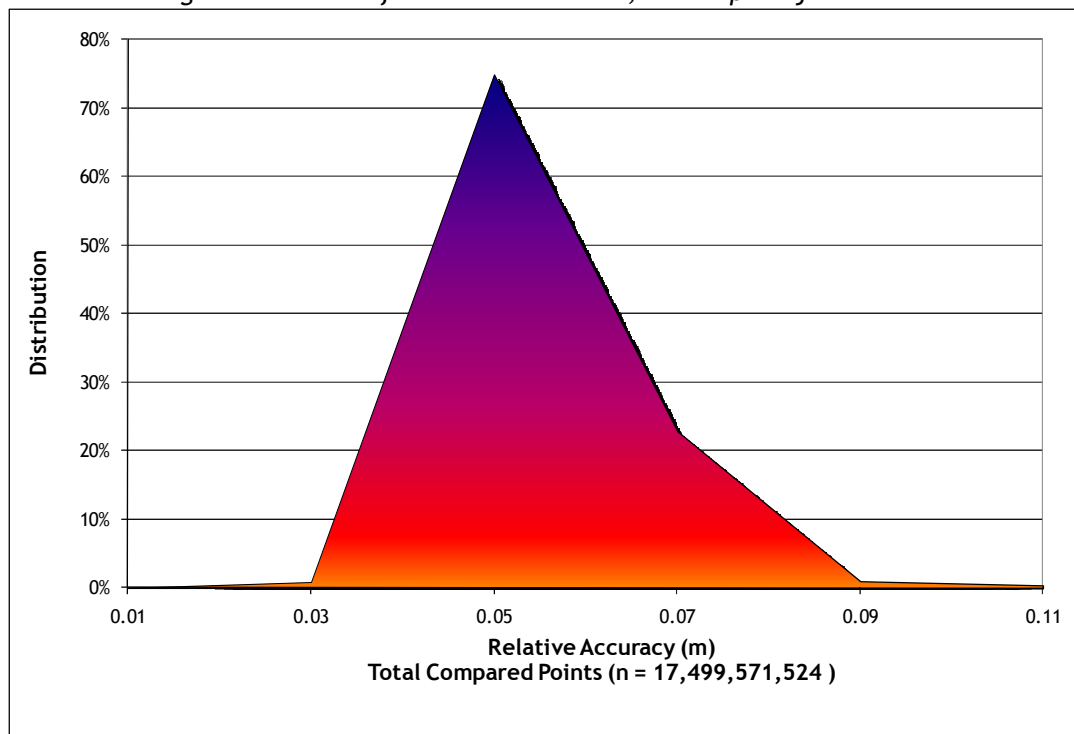
Figure 3.3. Percentage distribution of relative accuracies, non slope-adjusted.
