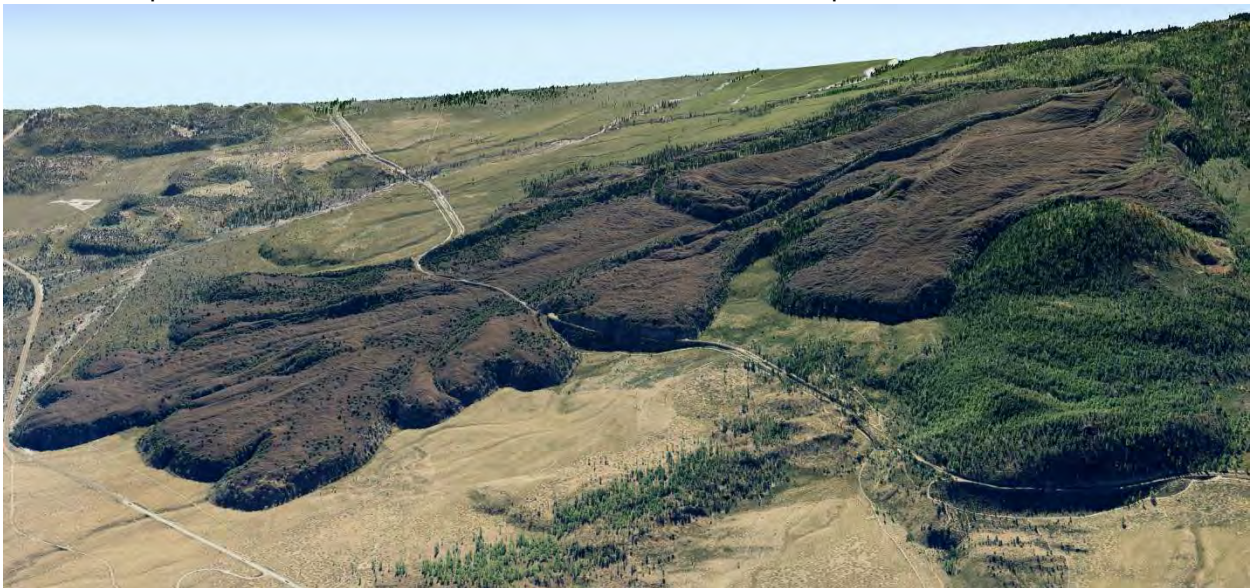
Figure 5.2. Lava flow on northern slope of Mount Shasta, view to the east. Image is a three dimensional point cloud with RGB values extracted from a NAIP orthophoto.
