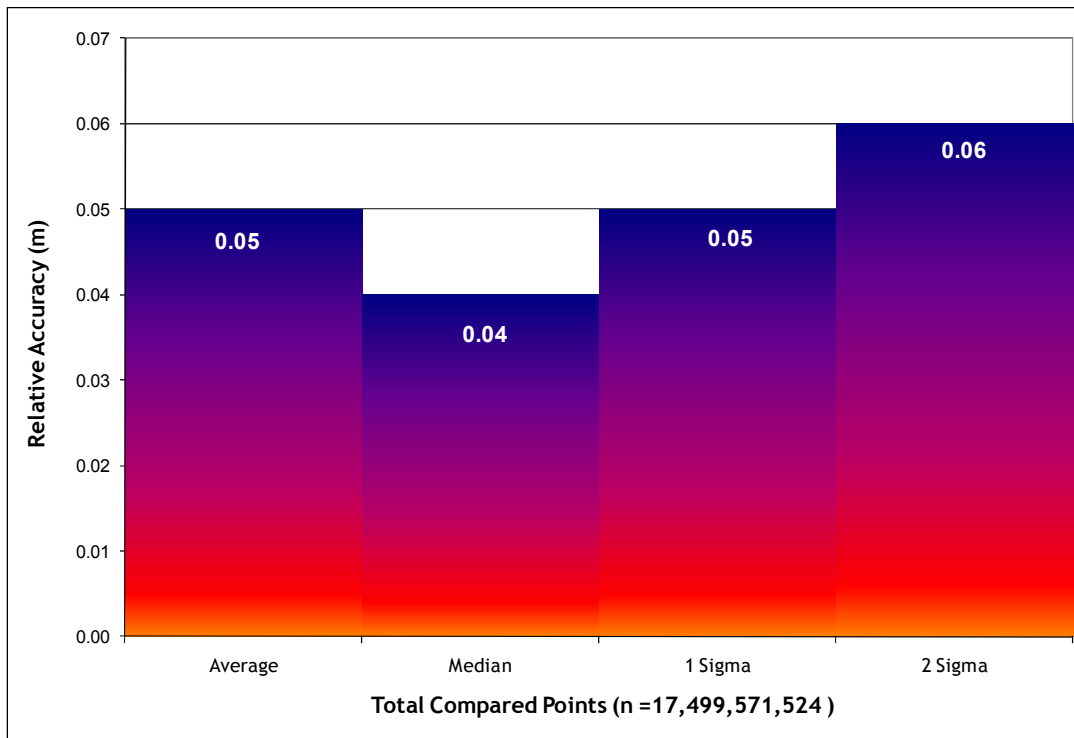
Figure 3.2. Statistical relative accuracies, non slope-adjusted.
