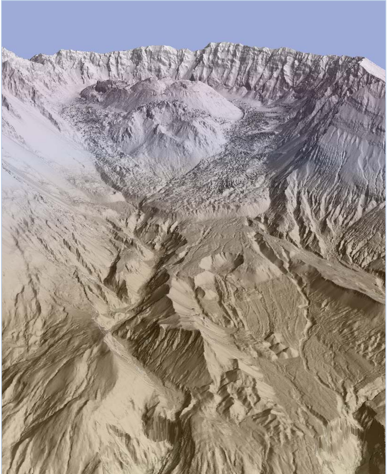
Figure 13. 3D view looking south into the crater of Mt St Helens (image is derived from ground-classified LiDAR points).
