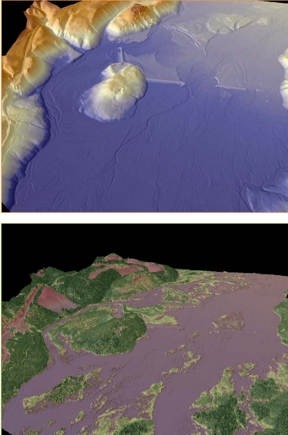
Figure 11. 3D views looking east northeast (slightly different vantage points) upstream along the Toutle River at the old Toutle Dam (center right) and debris dam site (upper center) along Hoffstadt Creek (top image is derived from ground-classified LiDAR points, and the bottom image is derived from highest-hit LiDAR points).
