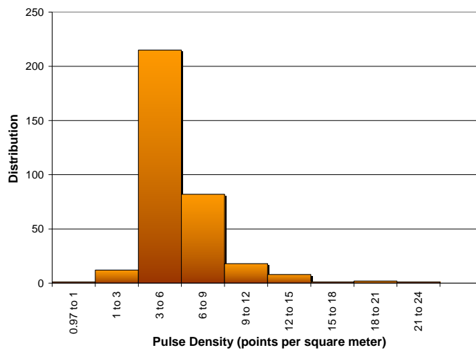
Figure 8. Ground-classified laser point data density.
