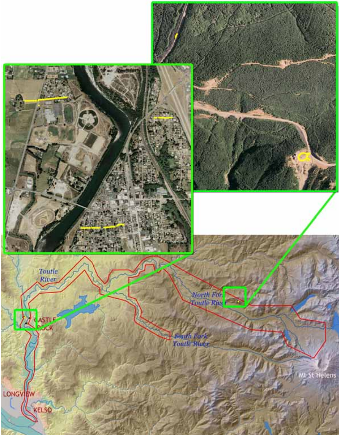
Figure 2. RTK and base station locations for study area.
