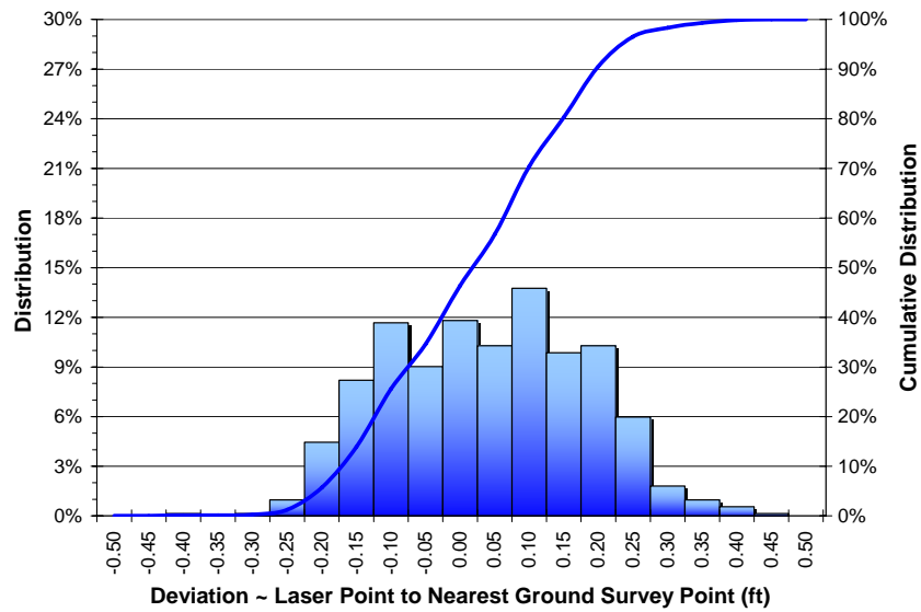
Figure 5. Absolute Accuracy Histogram Statistics
