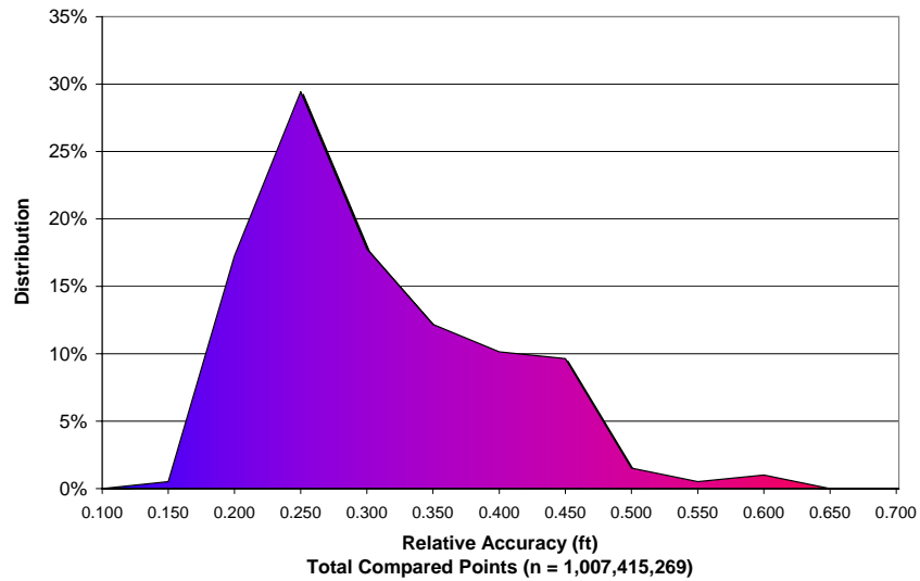
Figure 4. Statistical relative accuracies, non slope-adjusted.
