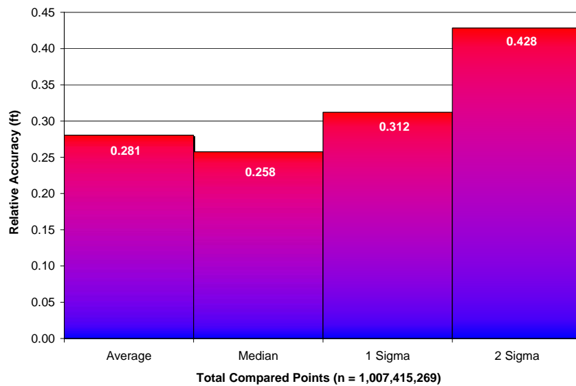
Figure 4. Statistical relative accuracies, non slope-adjusted.
