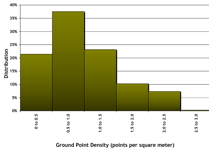
Figure 8. Ground-classified laser point data density.
