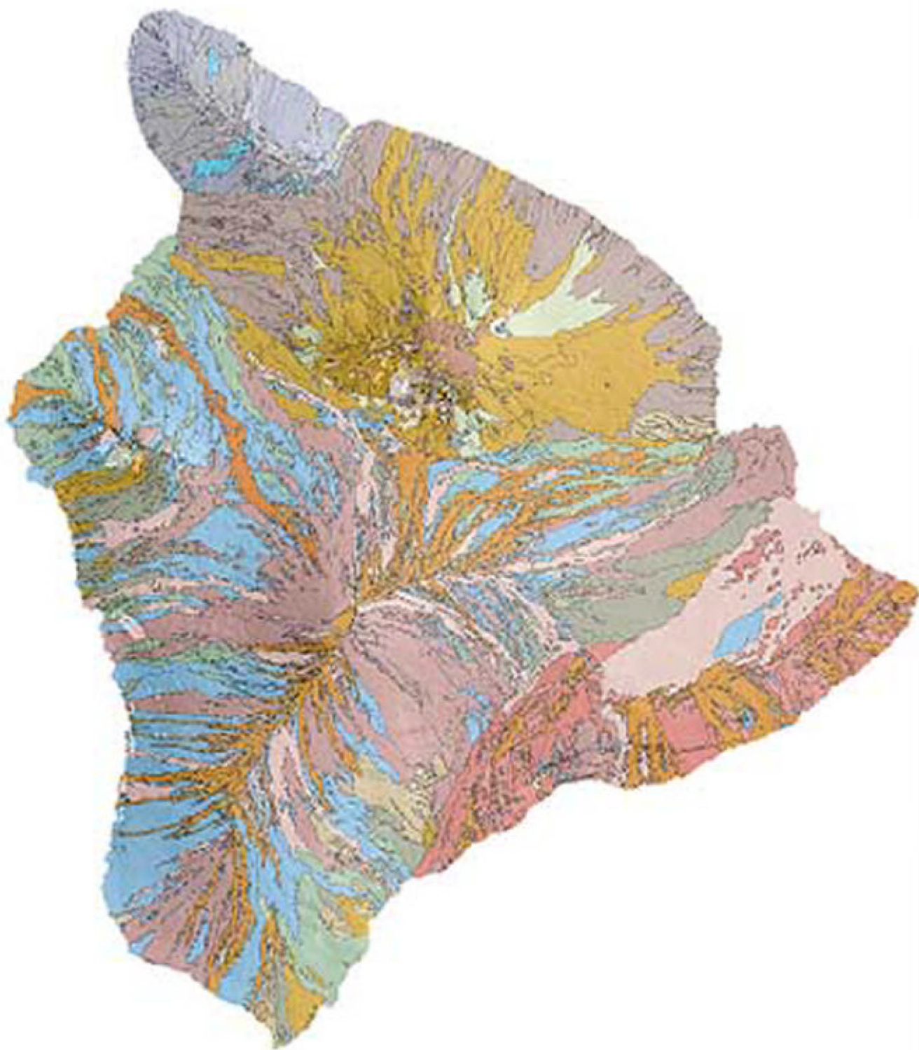
GEOLOGIC MAP OF THE ISLAND OF HAWAI'I
