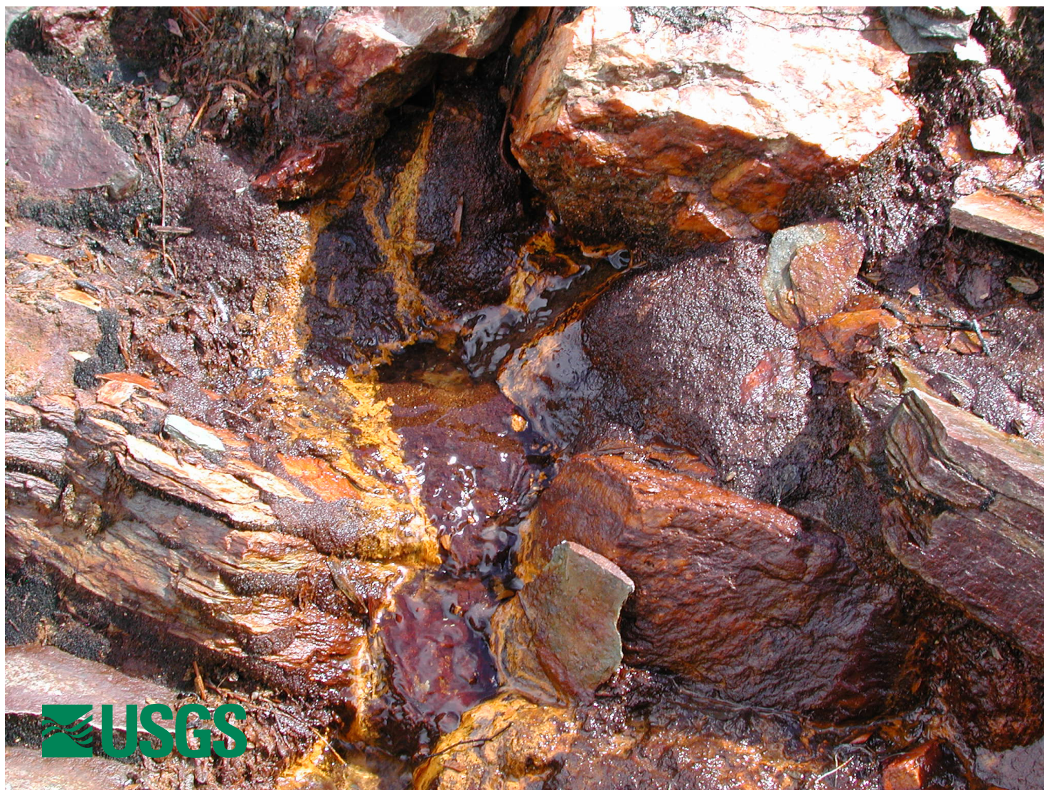
Photo 03BF008-7. Sampled spring at site with ferricrete.
