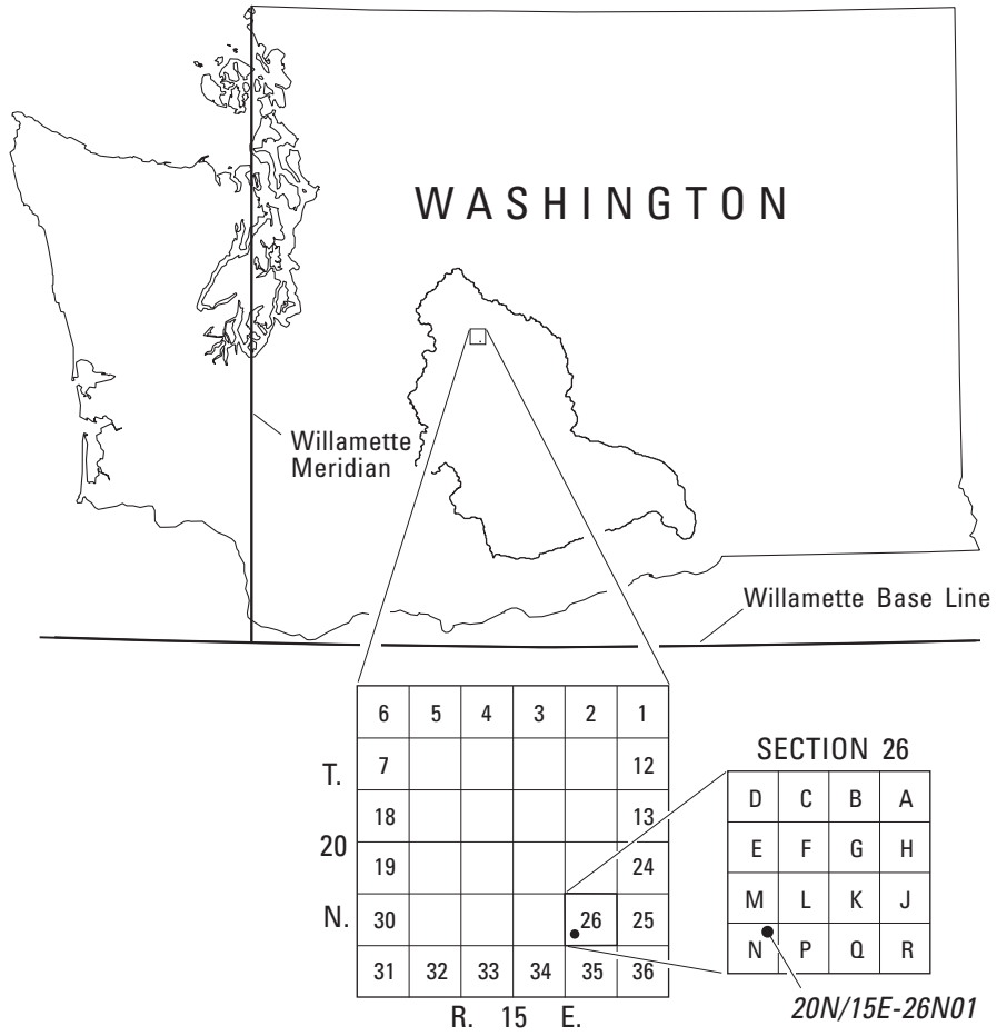
Figure 2. Well-numbering system used in the State of Washington.
