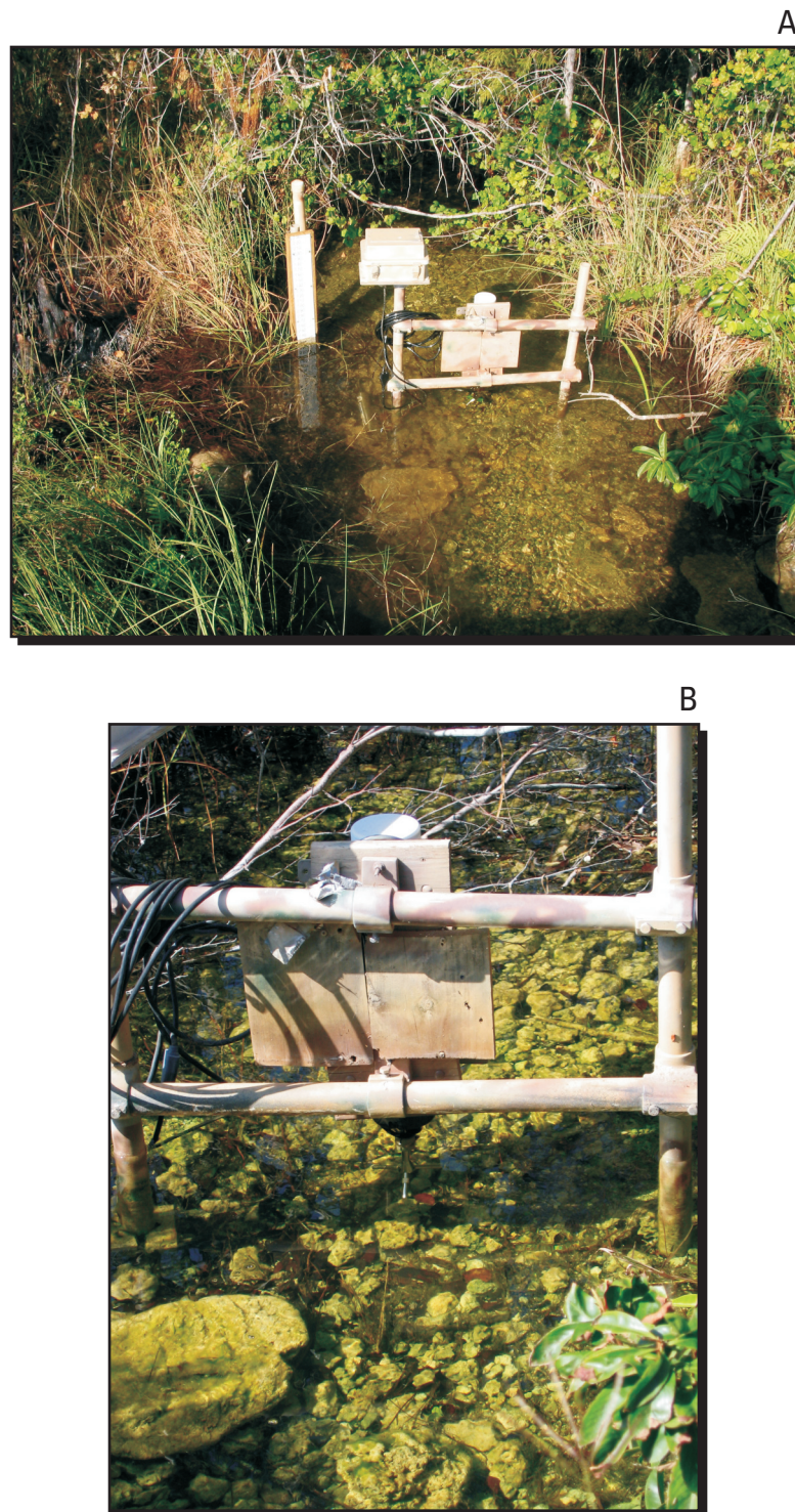
Figure 3. Distant and closeup views of the Argonaut-ADV® at (A) culvert 77 and (B) culvert 89. The ADV was in the middle of the piped mount system which created a rigid frame. The gray enclosure housed the communication cable. The Global Water pressure sensor was mounted to the PVC pipe shown in the background (see figure 5 for an enlarged view of this setup). The Sea-Bird conductivity meter was underwater on the left side next to the pipe.
