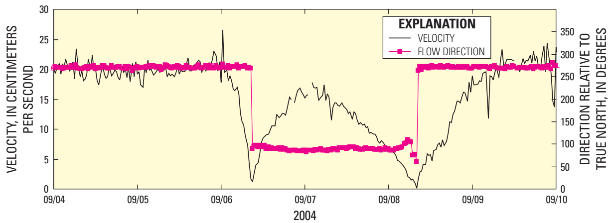
Figure 15. Flow-reversal event at culvert 77 during September 4-10, 2004.
