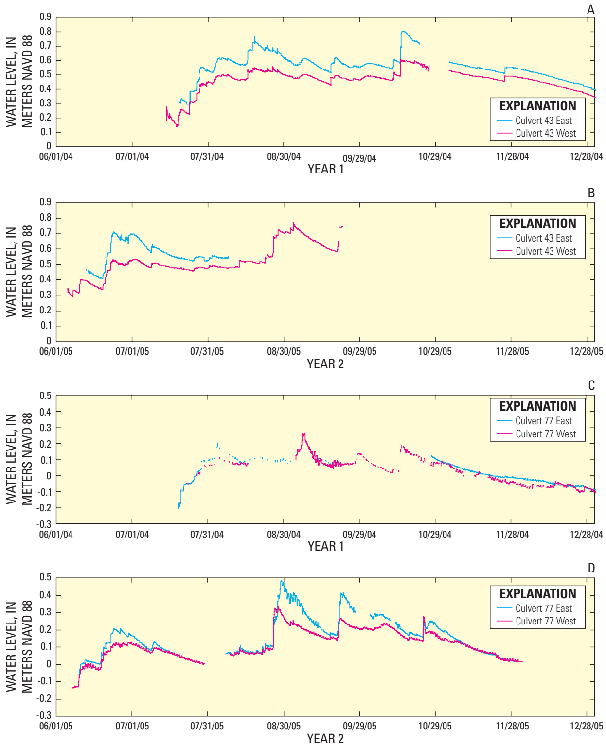
Figure 10. Water levels at culverts 43 and 77 during study years 1 and 2.
