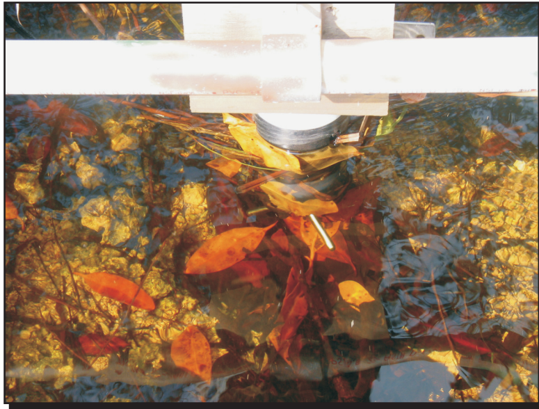
Figure 8. Leaves covering the Argonaut-ADV® transducer. Periods of missing data sometimes resulted from accumulations of vegetation, biological fouling, and wildlife interference of the instruments. The transducers (silver with a leaf on it) were just below the water surface.
