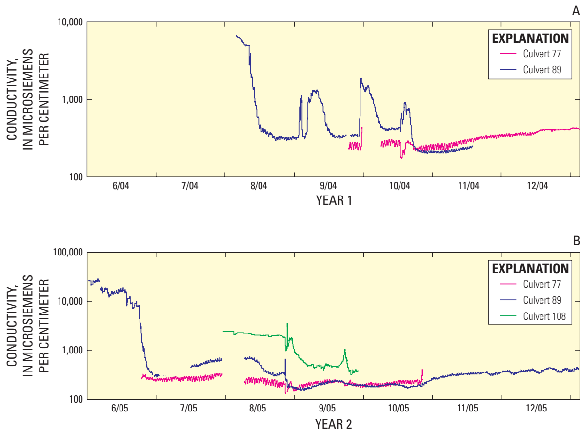
Figure 11. Conductivities at culverts 77, 89, and 108 during study years 1 and 2.
