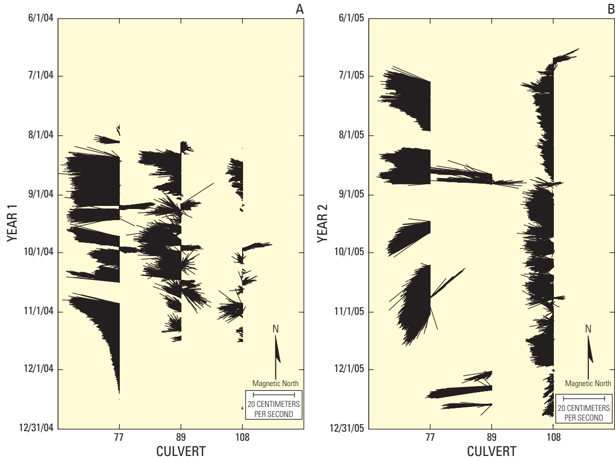
Figure 14. Flow velocities and flow directions at culverts 77, 89, and 108 during study years 1 and 2.
