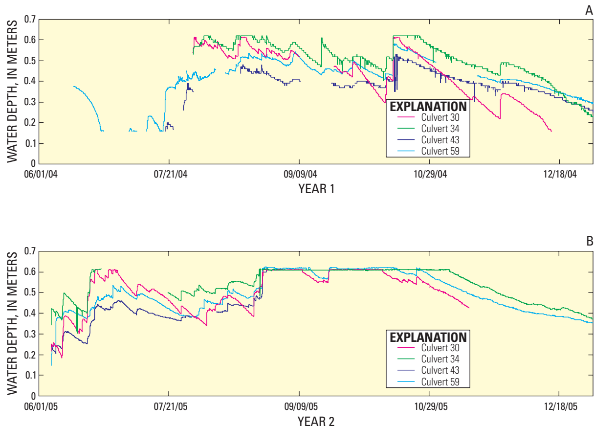
Figure 13. Recorded depth of water in culverts 30, 34, 43, and 59 during study years 1 and 2.
