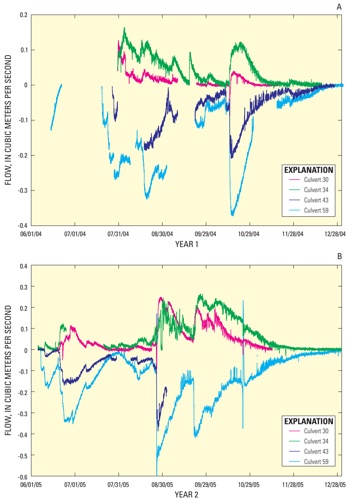
Figure 12. Computed discharge at culverts 30, 34, 43, and 59 during study years 1 and 2. Flows are positive for inflow to the Taylor Slough basin and negative for outflow toward Shark Slough basin during study years 1 and 2.
