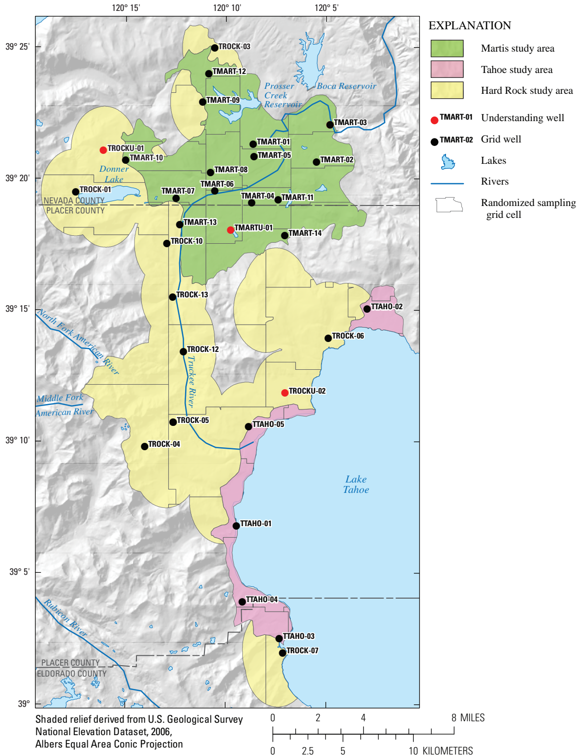
Figure 3. The northern (A) and southern (B) parts of the Tahoe–Martis Groundwater Ambient Monitoring and Assessment (GAMA) study unit, California, and the distribution of the study area grid cells, and locations of the sampled grid wells and the understanding wells.
