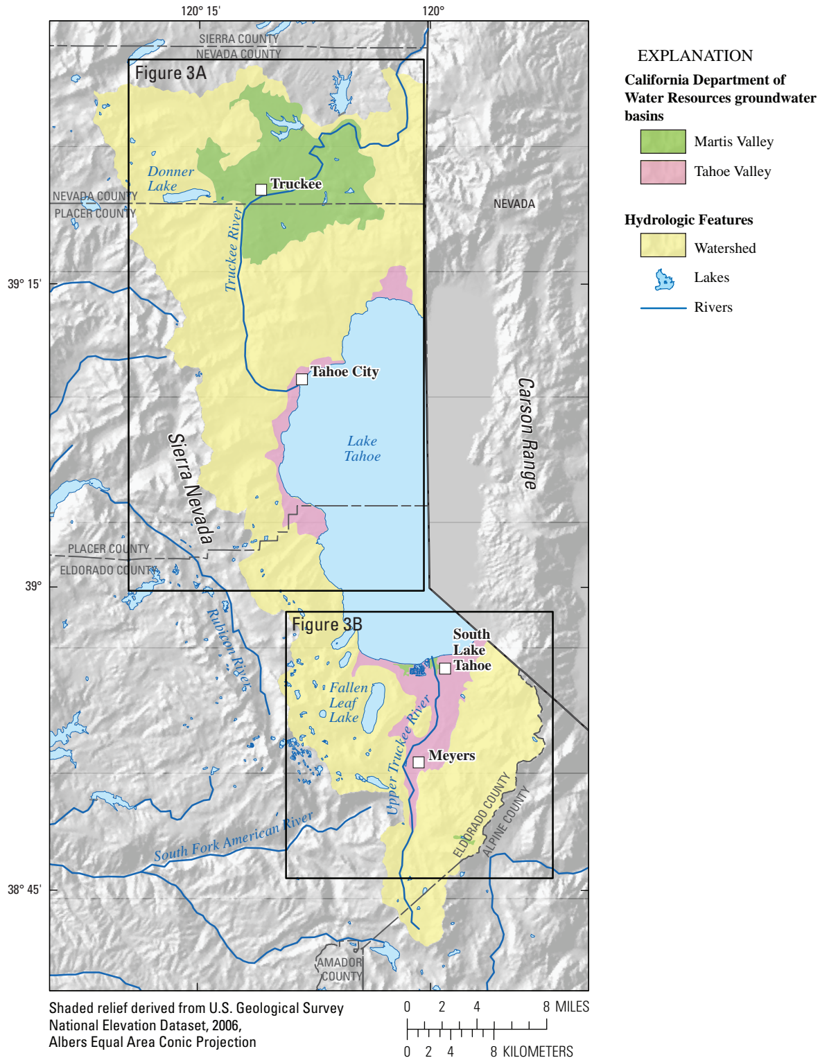
Figure 2. The Tahoe–Martis Groundwater Ambient Monitoring and Assessment (GAMA) study unit, and locations of groundwater basins, major cities, major hydrologic features, and the surface-water watershed area for Lake Tahoe and the Tahoe and Martis Valley groundwater basins, California.
