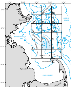
Location map outlining the 18 quadrangles in this series. Quadrangle 5 shown in blue. Stellwagen Bank National Marine Sanctuary (SBNMS) boundary indicated by dashed line. Bathymetric contours in meters.
