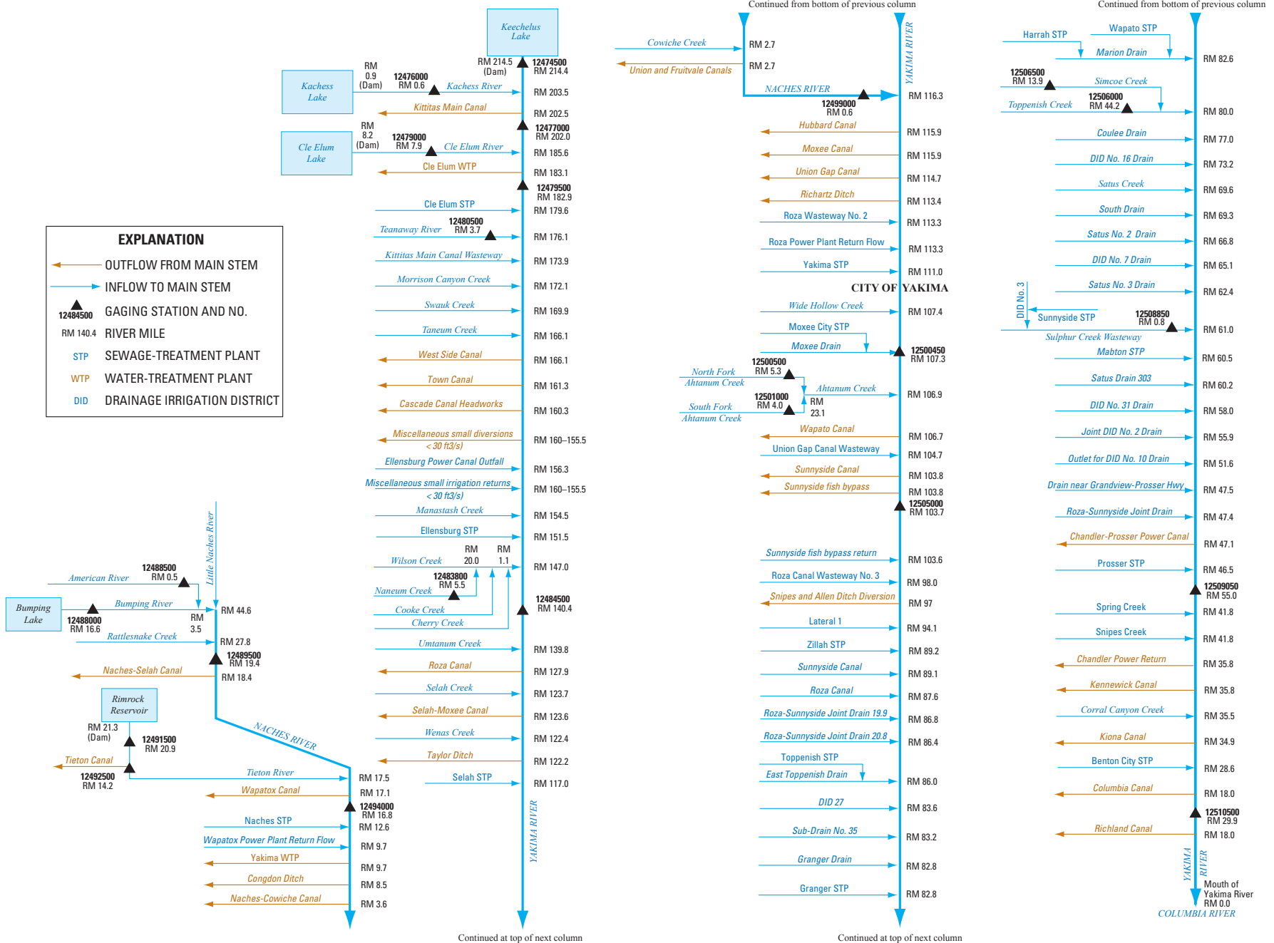
Figure 1. Selected tributaries, diversion canals, return flows, and streamflow-gaging stations, Yakima River basin, Washington.
