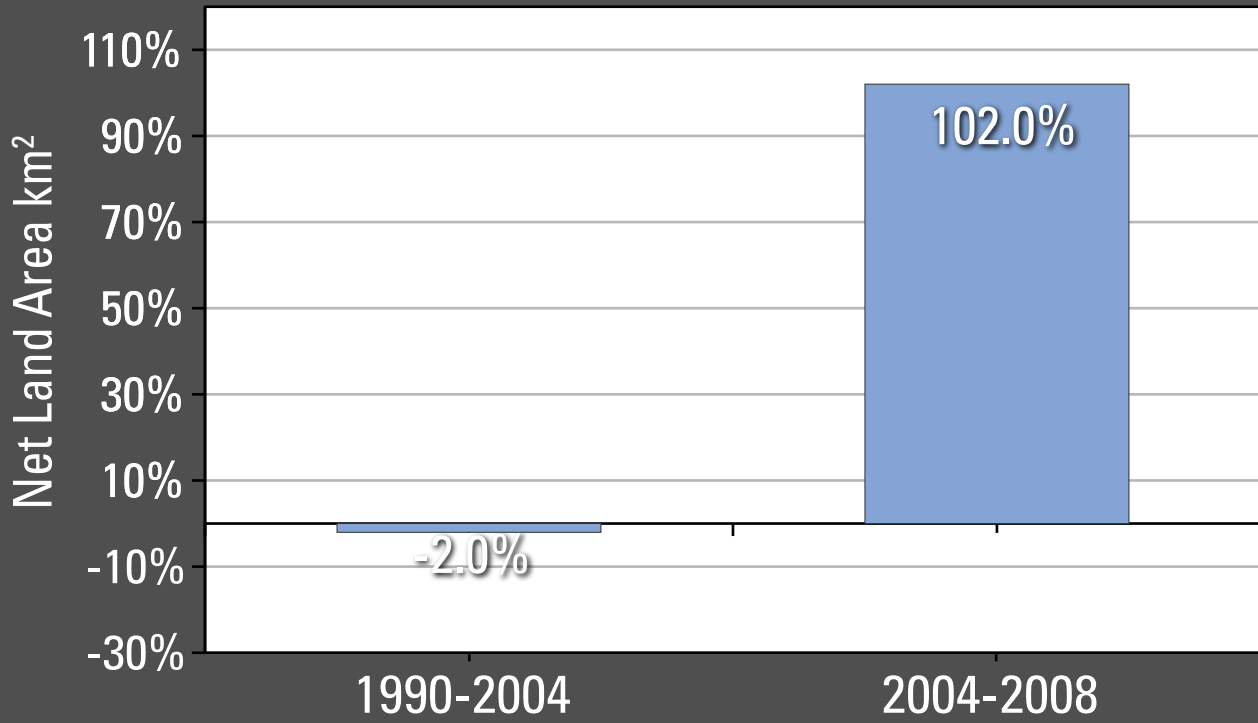
Figure 2. Percent net land loss from 1956 to 2004 and from 2004 to 2008 for Port Arthur, Texas.
