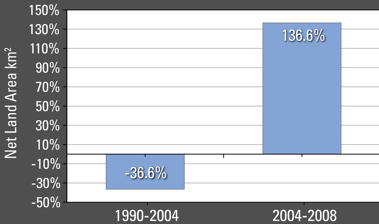
Figure 4. Net land area trends from 1990 to 2008 for the Blind Lake area, Texas.
