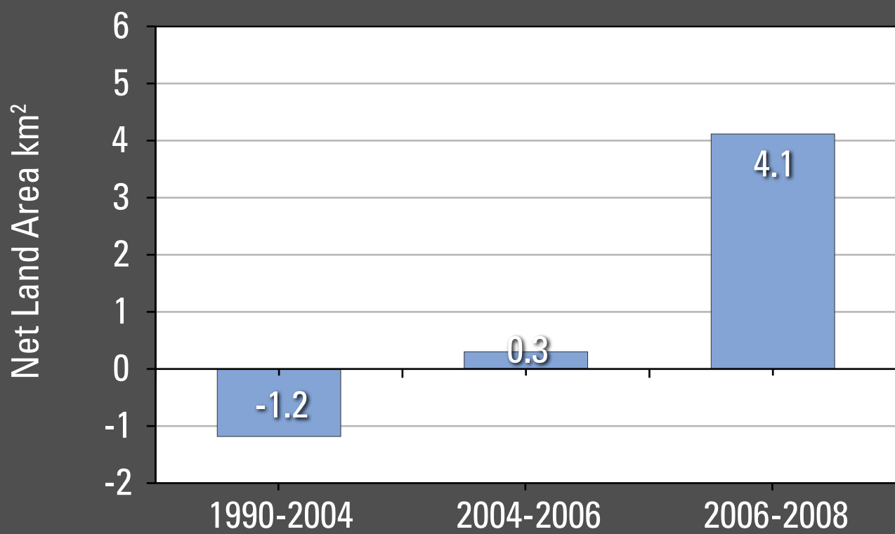
Figure 3. Net land area trends from 1990 to 2008 for the Blind Lake area, Texas.
