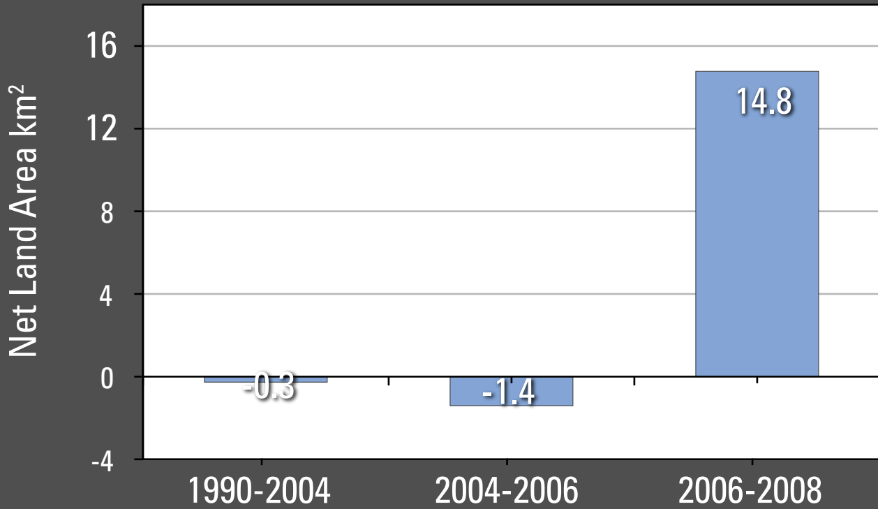
Figure 1. Net land area trends from 1990 to 2008 for Port Arthur, Texas.
