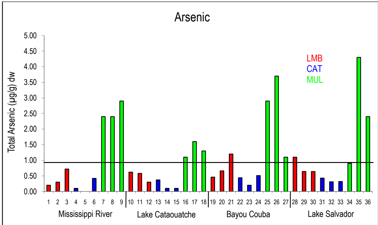
Figure 10A. Arsenic in dry weight from largemouth bass (LMB; Micropterus salmoides ), blue catfish (CAT; Ictalurus furcatus ), and striped mullet (MUL; Mugil cephalus ) collected from Davis Pond postdiversion sites from December 2007 through February 2009. The lower detection limit was 0.1 parts per million. The horizontal line represents the 85th percentile in dry weight from the National Contaminant Biomonitoring Program (Schmitt and Brumbaugh, 1990); for arsenic it is 0.93 micrograms per gram ( \mu\text{g/g} ).
