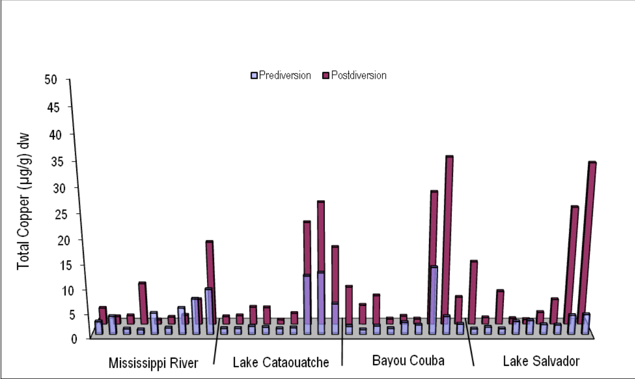
Figure 15B. Three-dimensional comparison of Davis Pond prediversion and postdiversion values for copper by dry weight (in micrograms per gram [µg/g]).
