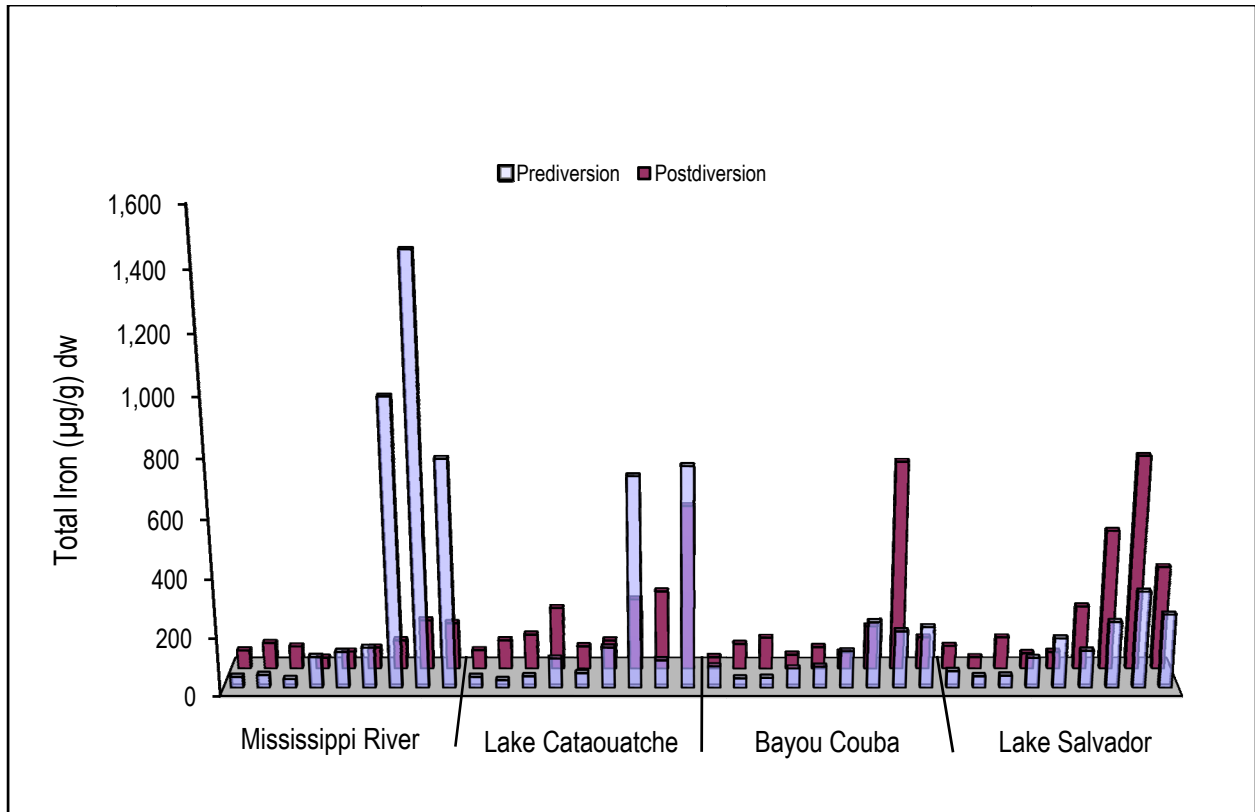
Figure 16B. Three-dimensional comparison of Davis Pond prediversion and postdiversion values for iron by dry weight (in micrograms per gram [µg/g]).
