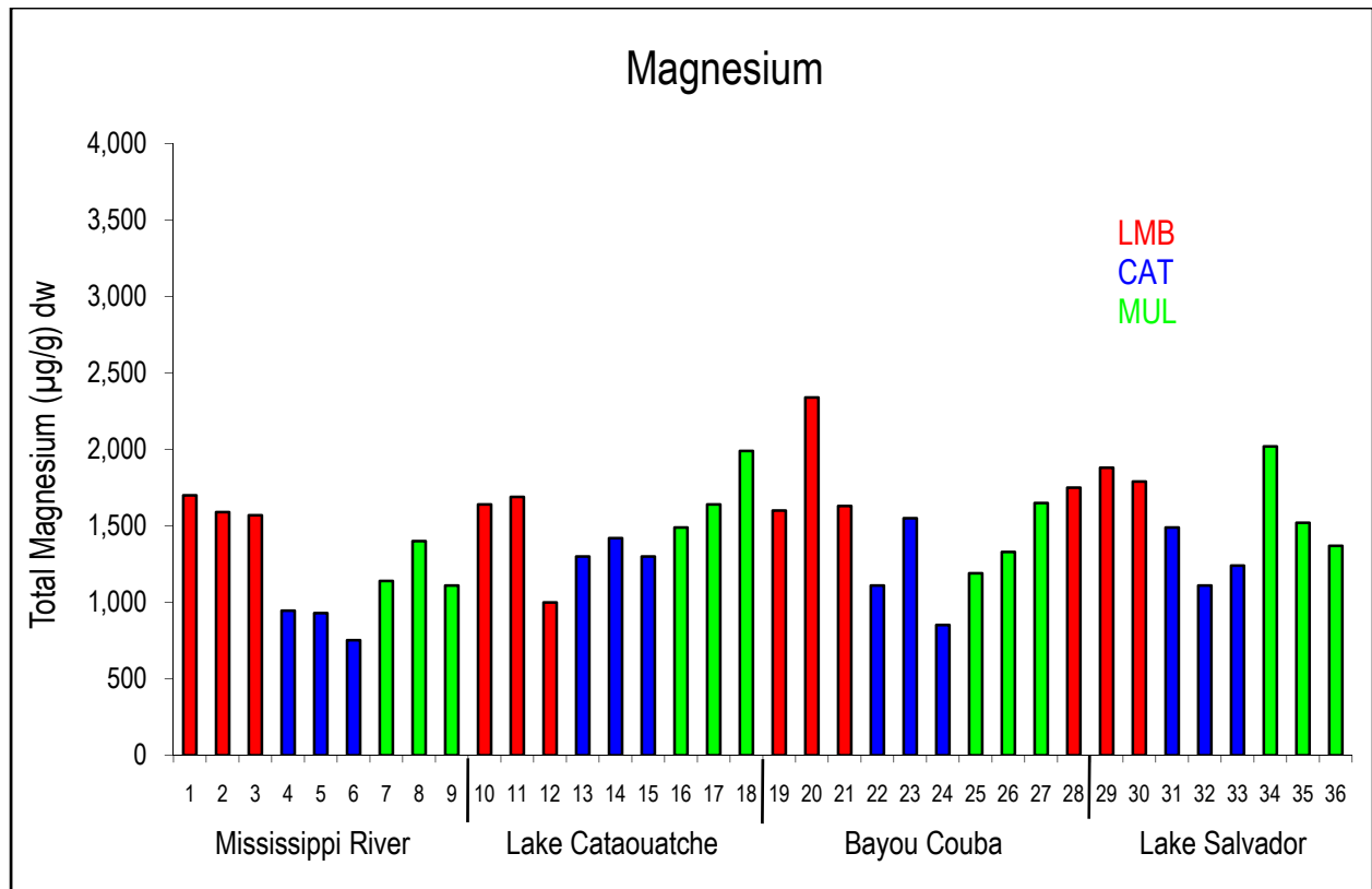
Figure 18A. Magnesium in dry weight from largemouth bass (LMB; Micropterus salmoides ), blue catfish (CAT; Ictalurus furcatus ), and striped mullet (MUL; Mugil cephalus ) collected from Davis Pond postdiversion sites from December 2007 through February 2009.
