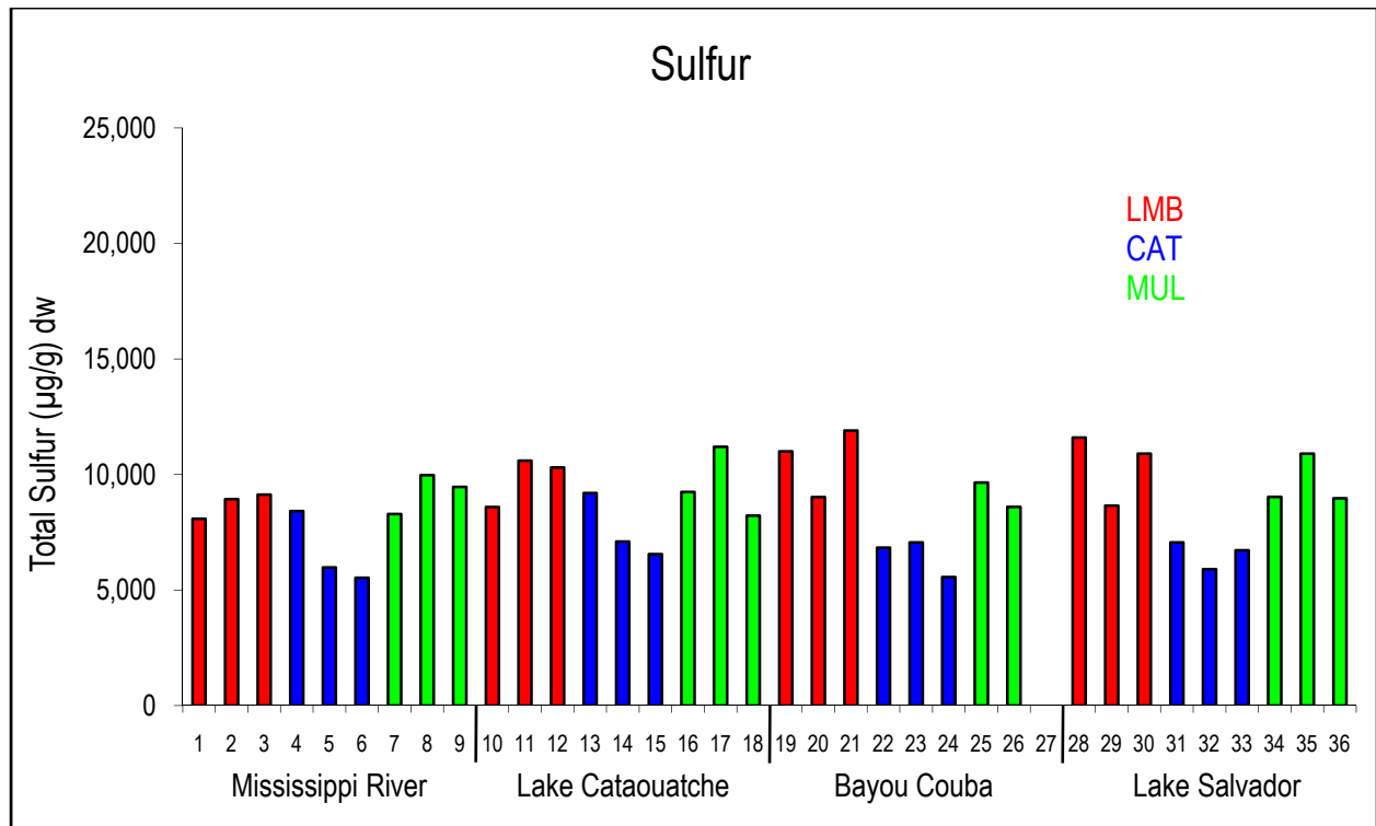
Figure 24A. Sulfur in dry weight from largemouth bass (LMB; Micropterus salmoides ), blue catfish (CAT; Ictalurus furcatus ), and striped mullet (MUL; Mugil cephalus ) collected from Davis Pond postdiversion sites from December 2007 through February 2009.
