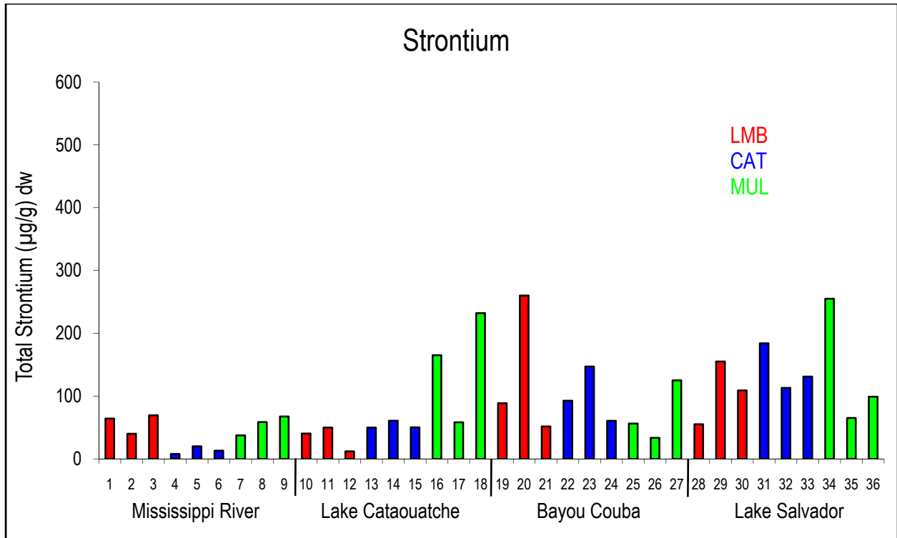
Figure 25A. Strontium in dry weight from largemouth bass (LMB; Micropterus salmoides ), blue catfish (CAT; Ictalurus furcatus ), and striped mullet (MUL; Mugil cephalus ) collected from Davis Pond postdiversion sites from December 2007 through February 2009.
