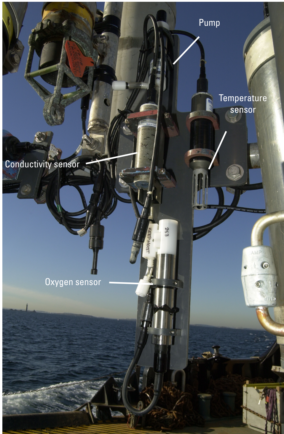
Figure 17. Sea-Bird oxygen, conductivity, and temperature sensors and pump mounted on tripod frame (shown in fig. 4A). Photograph by Dann Blackwood, U.S. Geological Survey.
