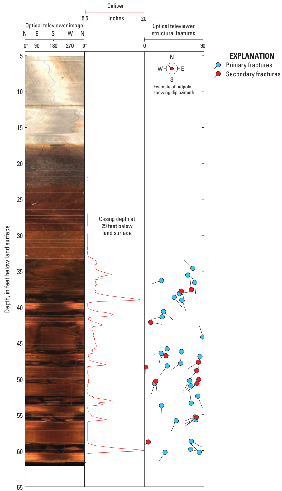
Appendix 5-6. Optical televiewer images and structural orientations of foliation, lithologic contacts, and fractures in well PS-098.
