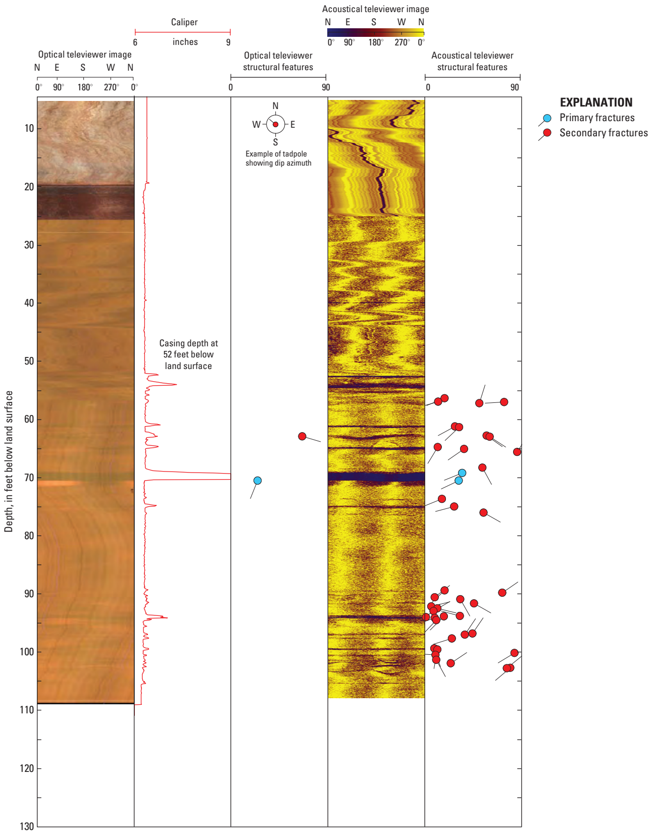
Appendix 5-15. Optical and acoustical televiwer images and structural orientations of fractures in well PS-107.
