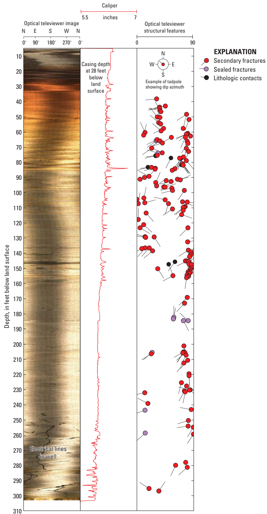
Appendix 5-3. Optical televiewer images and structural orientations of foliation, lithologic contacts, and fractures in well PS-095.
