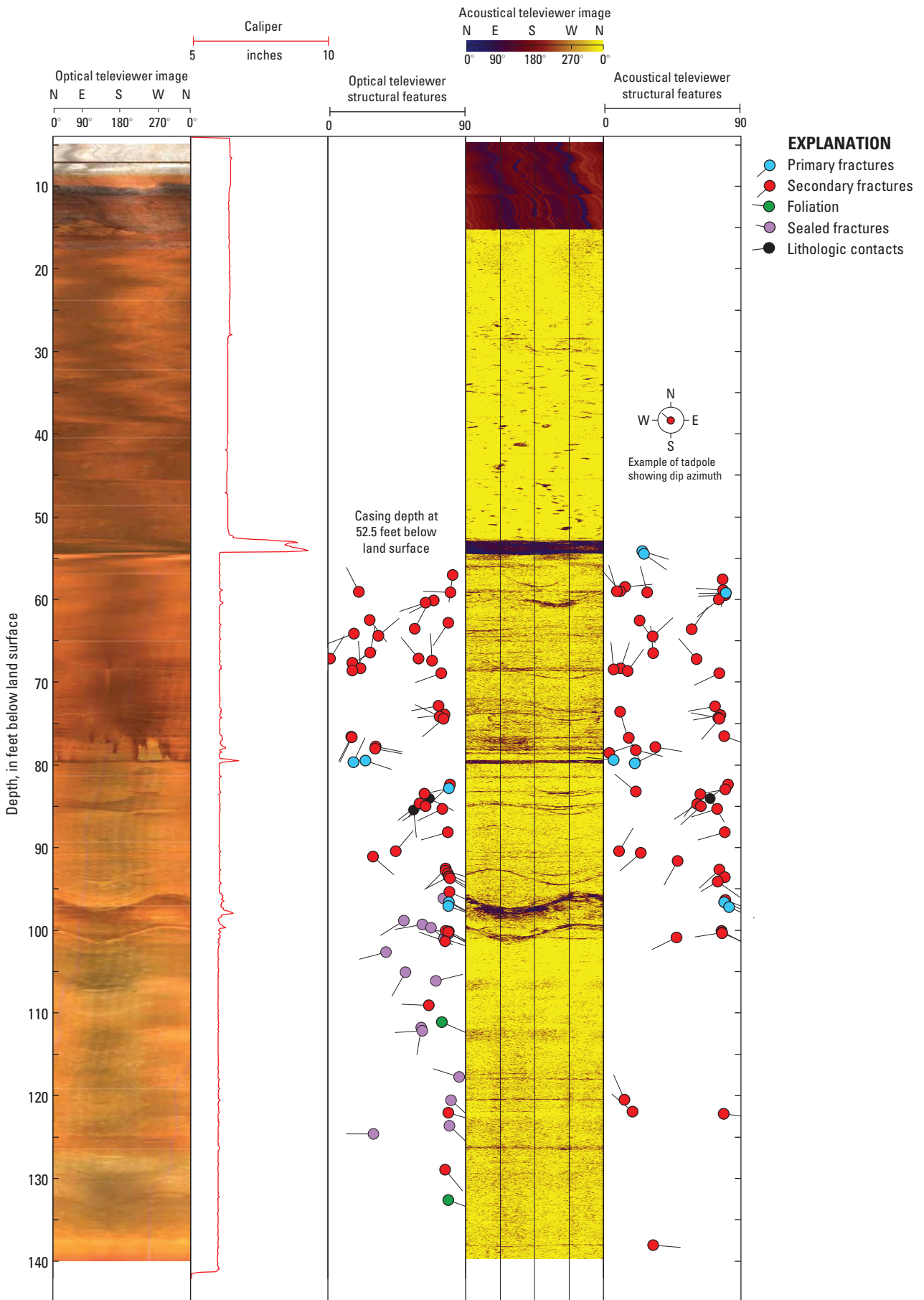
Appendix 5-5. Optical and acoustical televiwer images and structural orientations of primary and secondary fractures in well PS-097.
