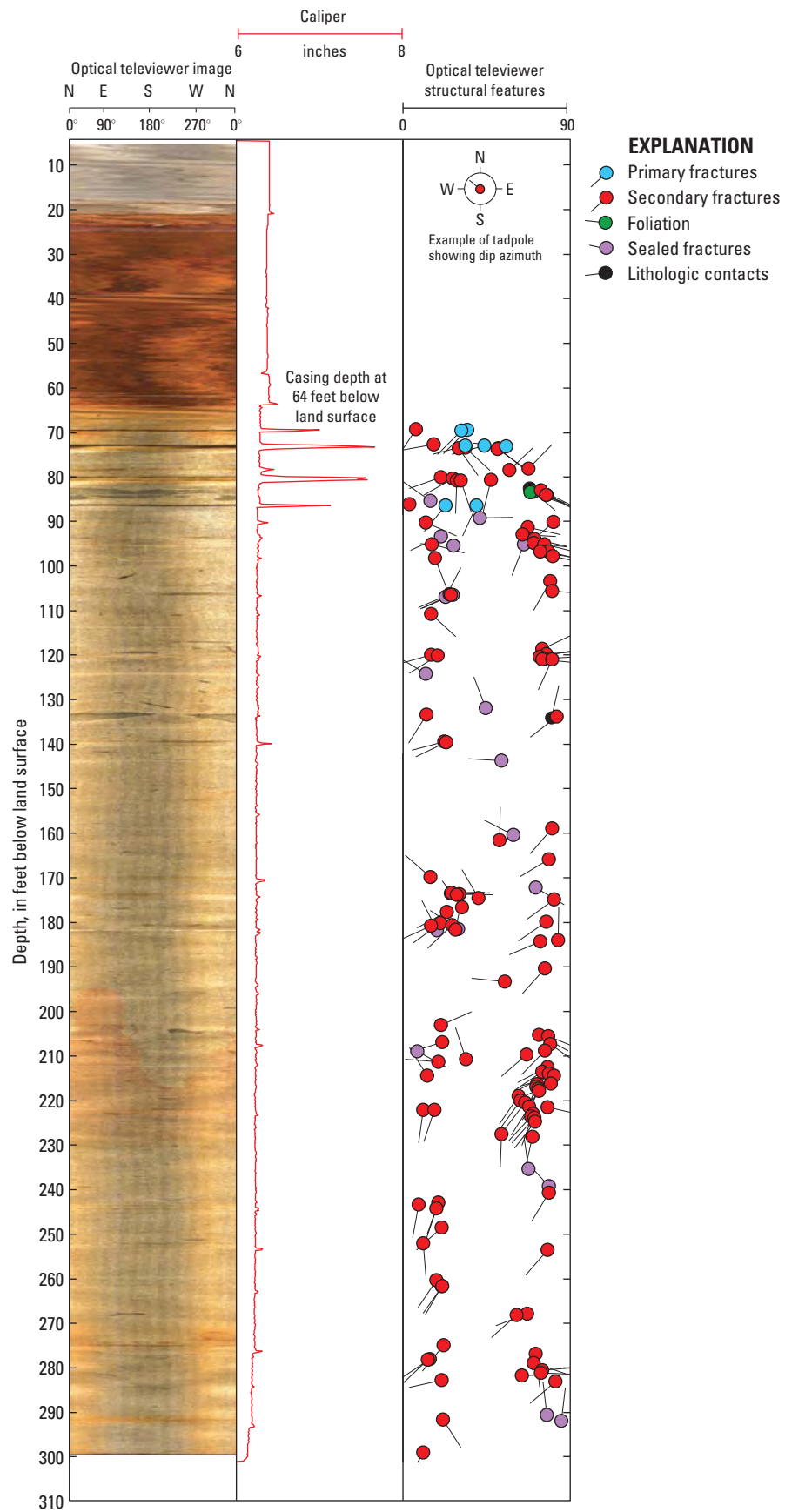
Appendix 5-7. Optical televiewer images and structural orientations of foliation, lithologic contacts, and fractures in well PS-099.
