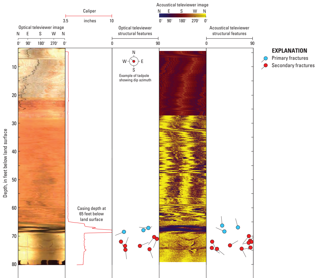
Appendix 5-12. Optical and acoustical televiwer images and structural orientations of foliation, lithologic contacts, and fractures in well PS-104.
