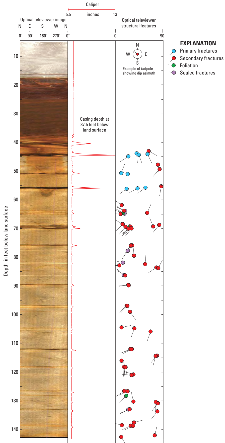
Appendix 5-8. Optical televiewer images and structural orientations of foliation, lithologic contacts, and fractures in well PS-100.
