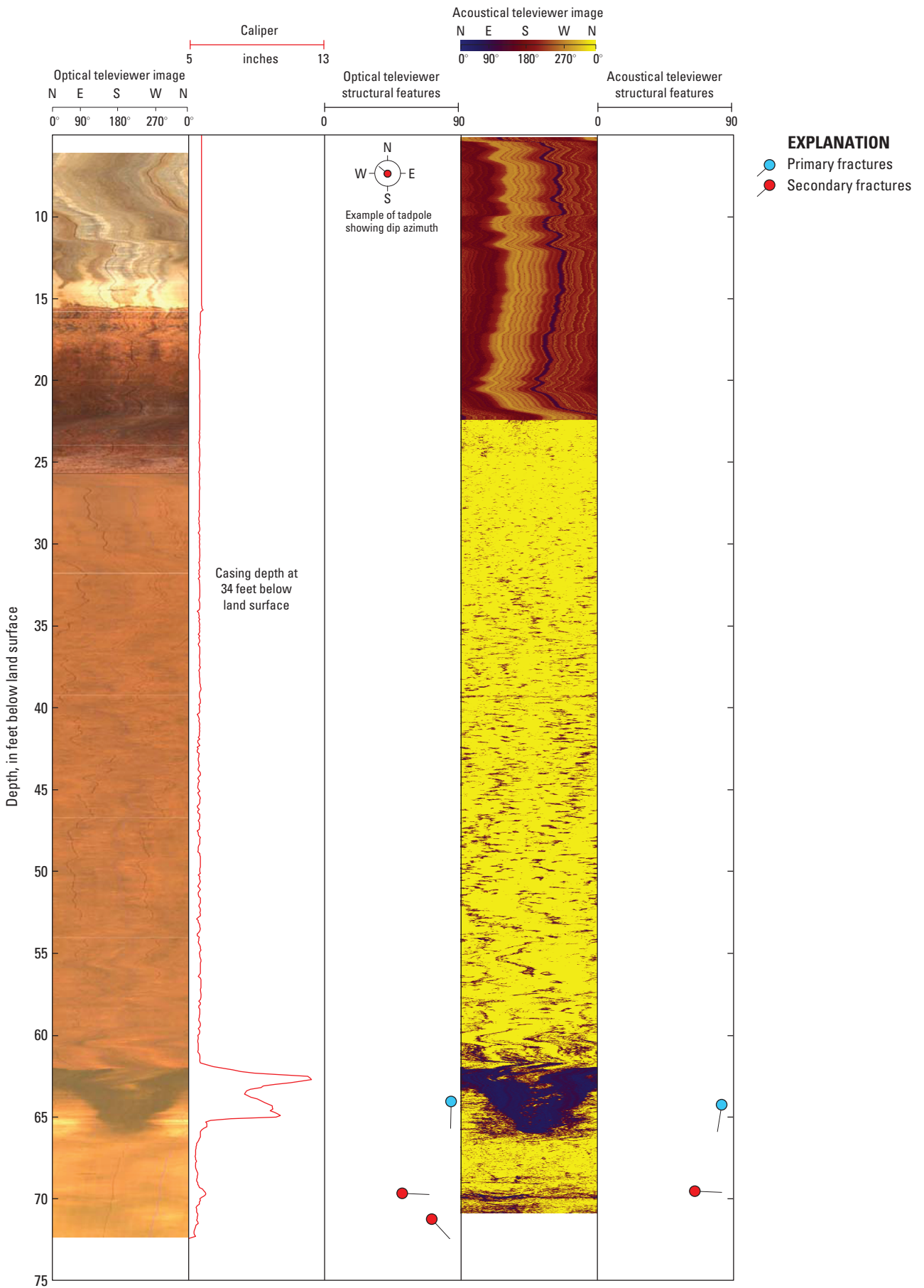
Appendix 5-4. Optical and acoustical televIEWER images and structural orientations of primary and secondary fractures in well PS-096.
