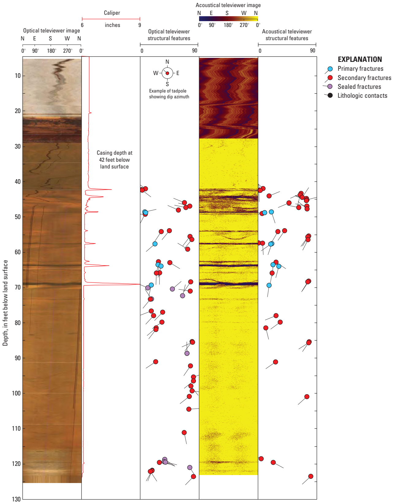
Appendix 5-2. Optical and acoustical televiwer images and structural orientations of foliation, lithologic contacts, and fractures in well PS-094.
