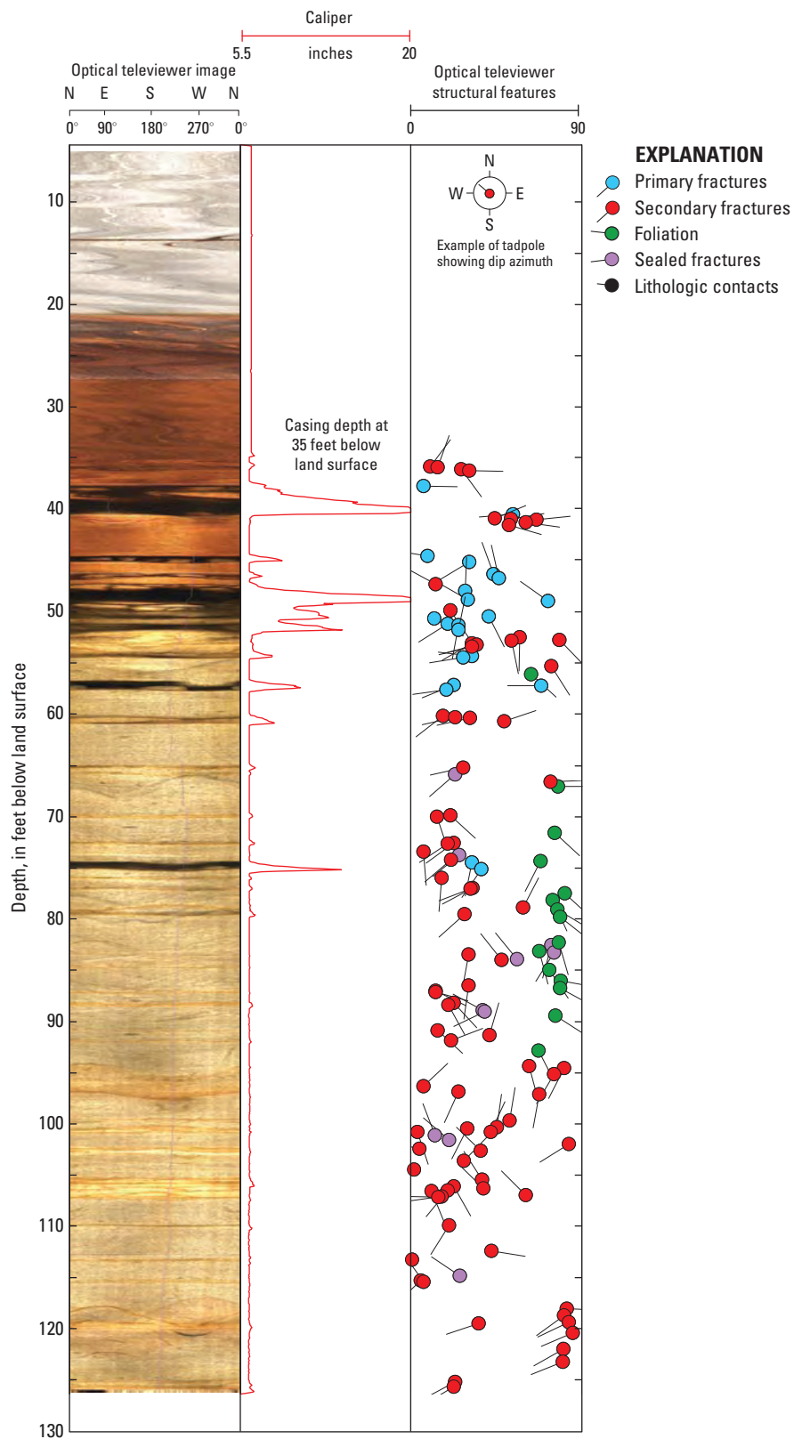
Appendix 5-14. Optical and acoustical televIEWER images and structural orientations of foliation, lithologic contacts, and fractures in well PS-106.
