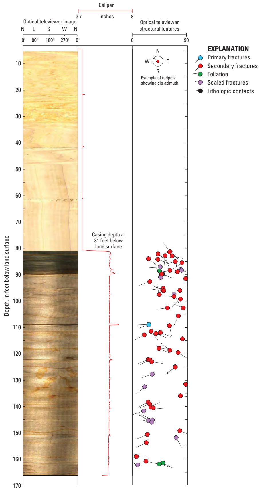
Figure 5-11. Optical televiewer images and structural orientations of foliation, lithologic contacts, and fractures in well PS-103.
