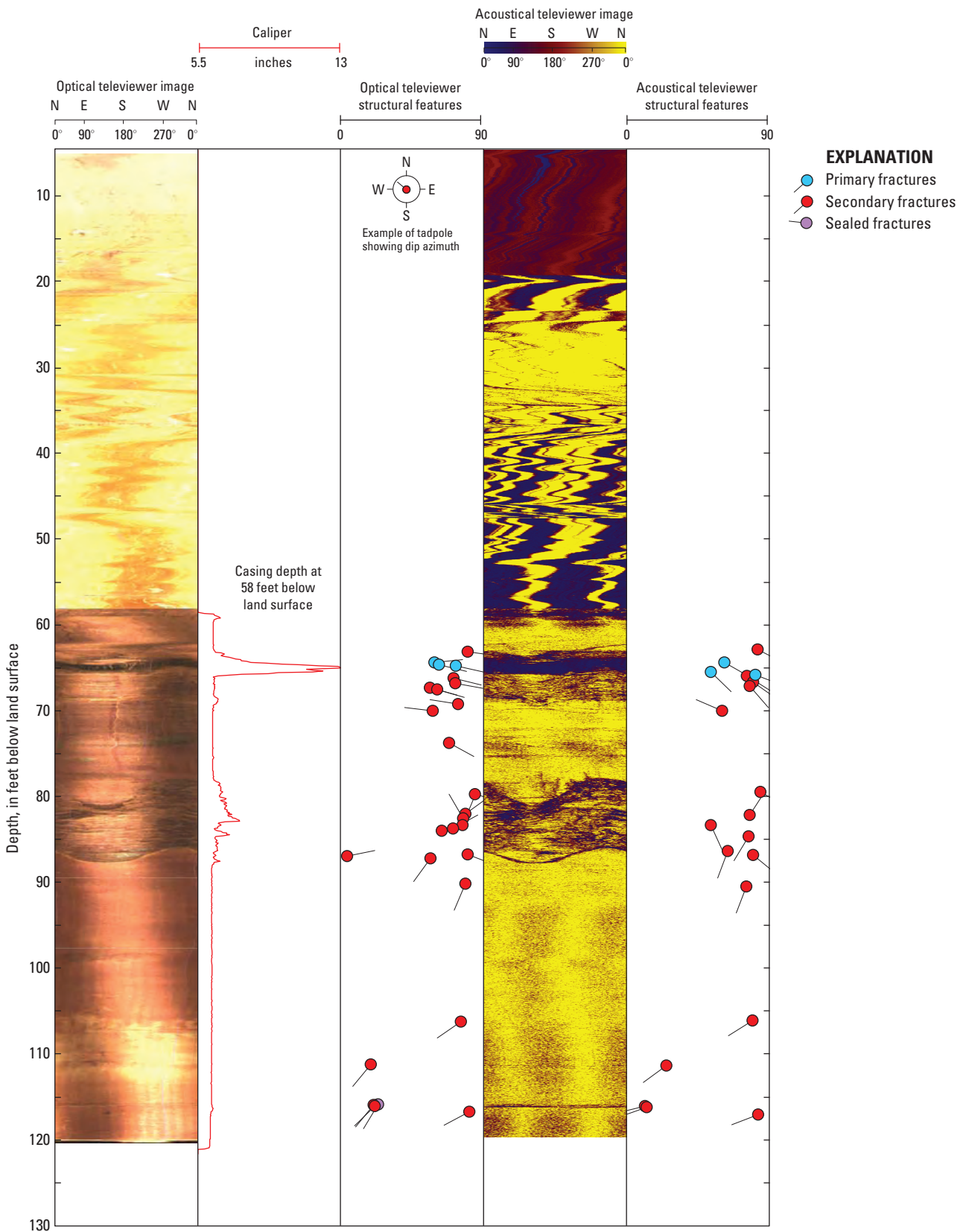
Appendix 5-10. Optical and acoustical televiwer images and structural orientations of foliation, lithologic contacts, and fractures in well PS-102.
