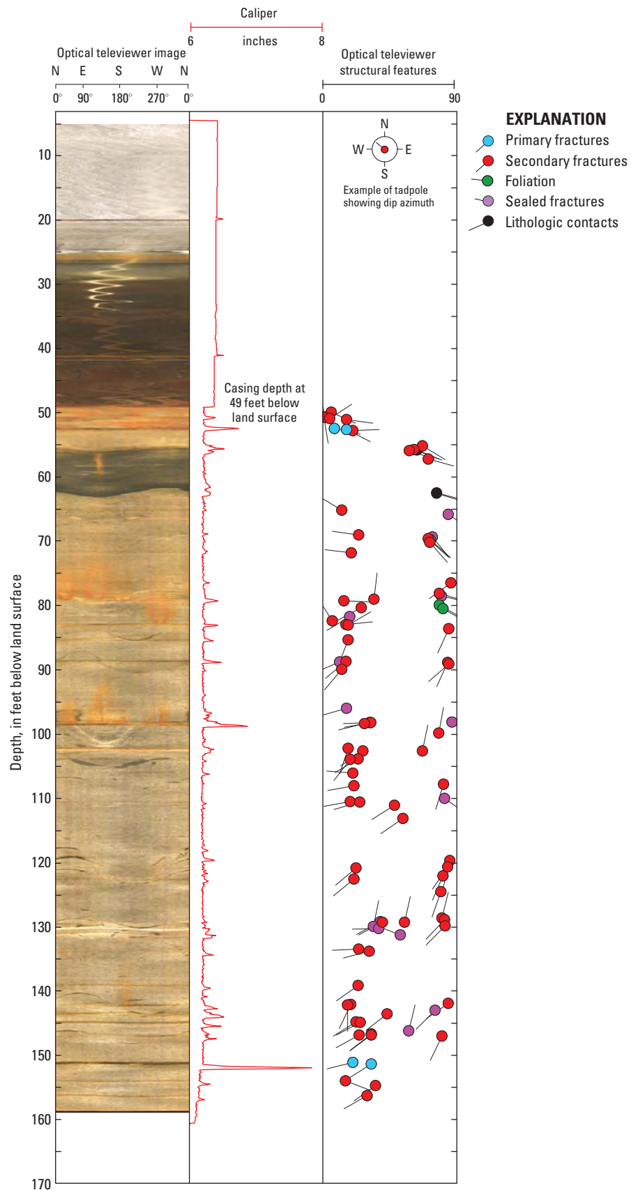
Appendix 5-13. Optical televiewer images and structural orientations of foliation, lithologic contacts, and fractures in well PS-105.
