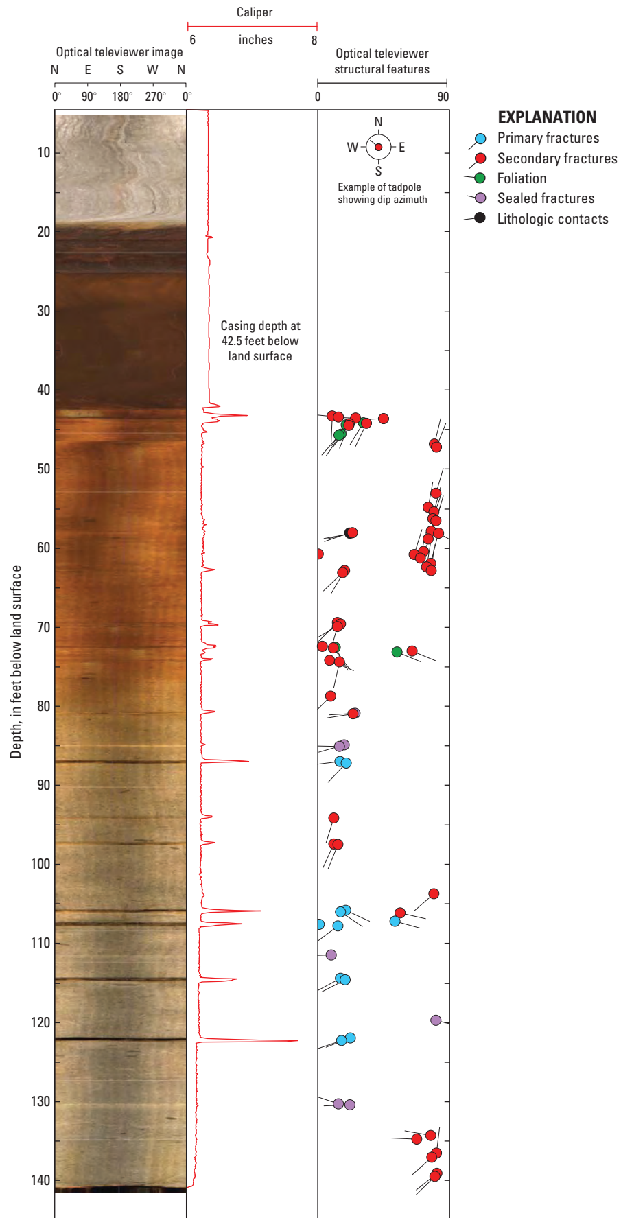
Appendix 5-1. Optical televiewer images and structural orientations of foliation, lithologic contacts, and fractures in well PS-093.
