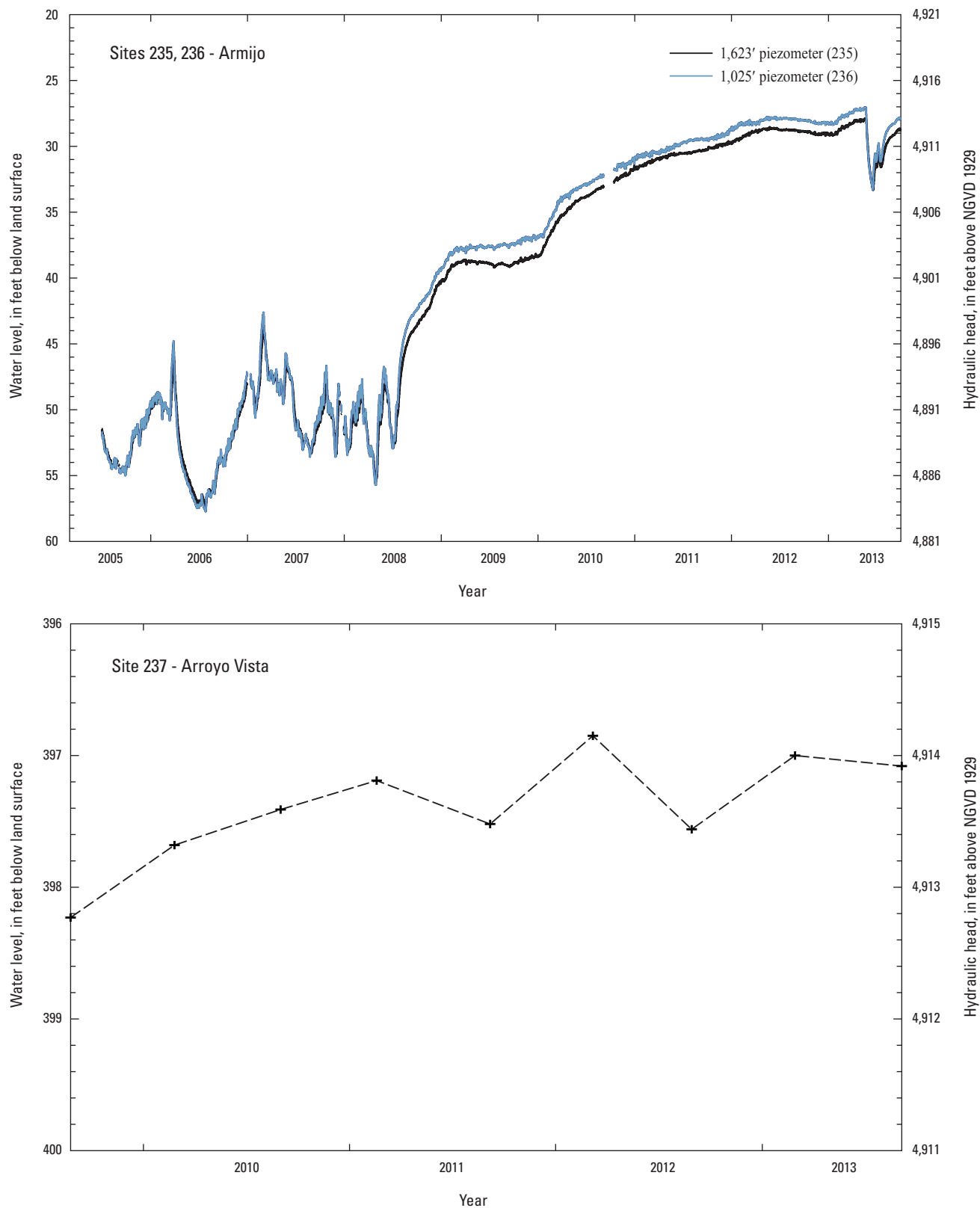
Figure 4. Water-level data for selected wells and piezometers in the Albuquerque Basin, central New Mexico.—Continued
