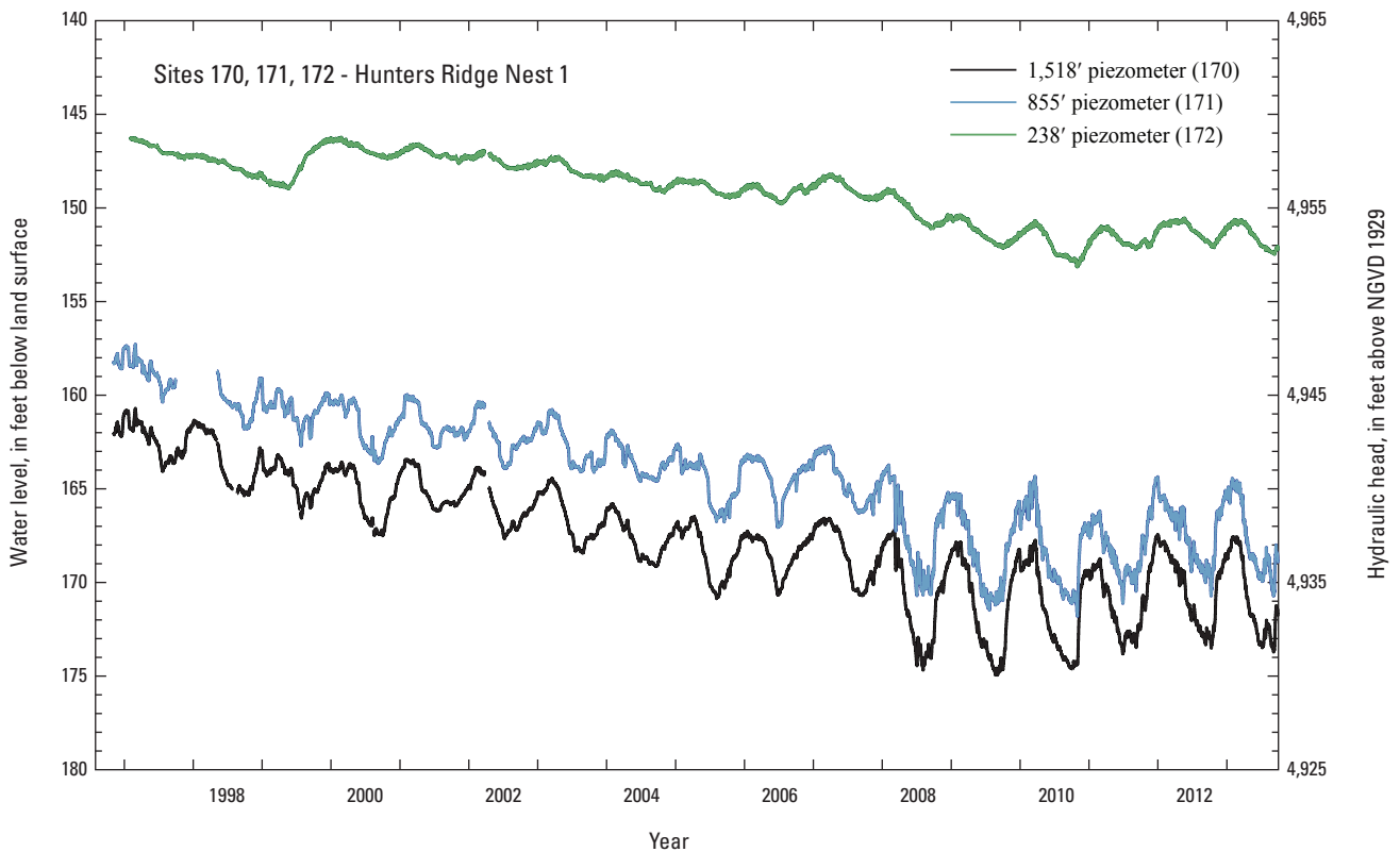
Figure 4. Water-level data for selected wells and piezometers in the Albuquerque Basin, central New Mexico.—Continued
