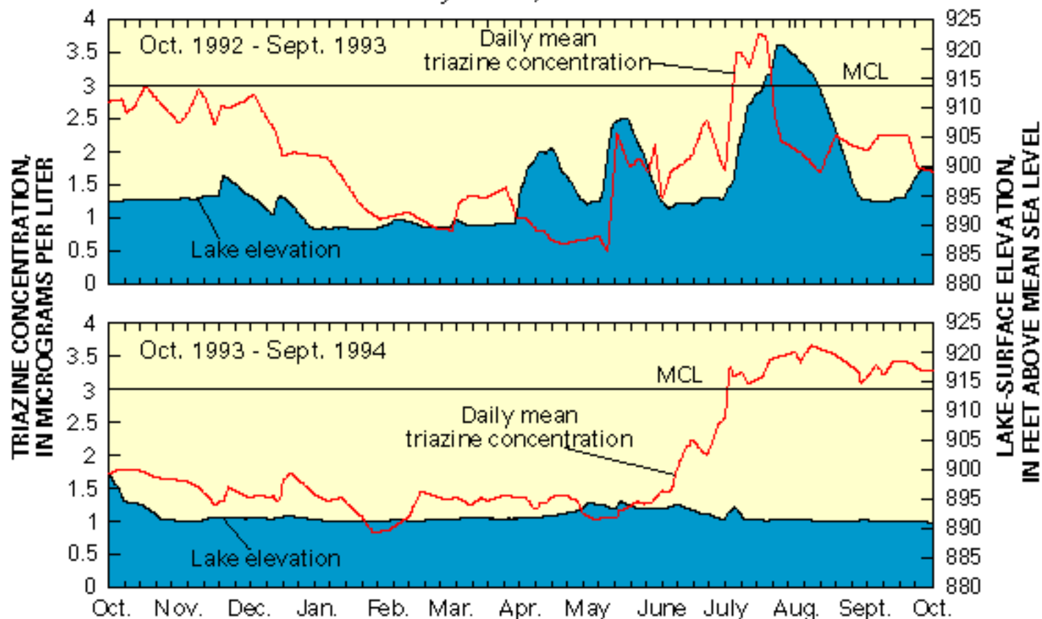
Figure 3. Daily mean triazine concentrations in the outflow to Perry Lake and lake-surface elevation (sampling site 11, fig. 1).
