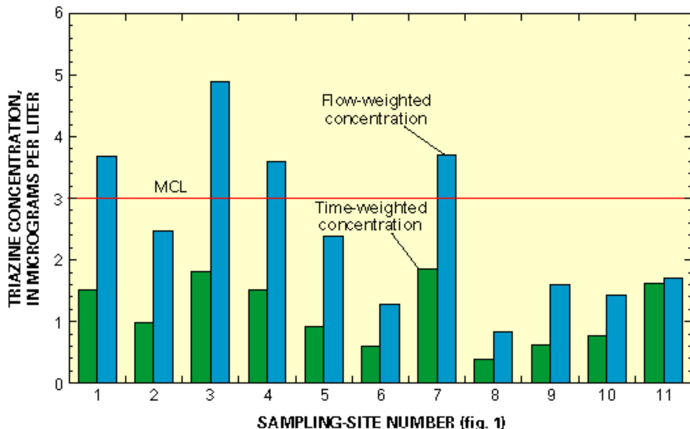
Figure 4. Time- and flow-weighted mean triazine concentrations for April 1, 1993, through March 31, 1994.
