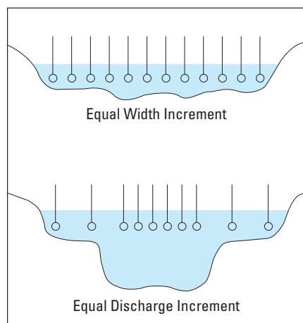
Figure 2. Methods for collecting samples in a cross section of a stream with shallow even flow and deep channelized flow.
