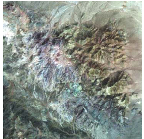
Landsat 7 ETM+ FCC of the Drum Mts., Utah
