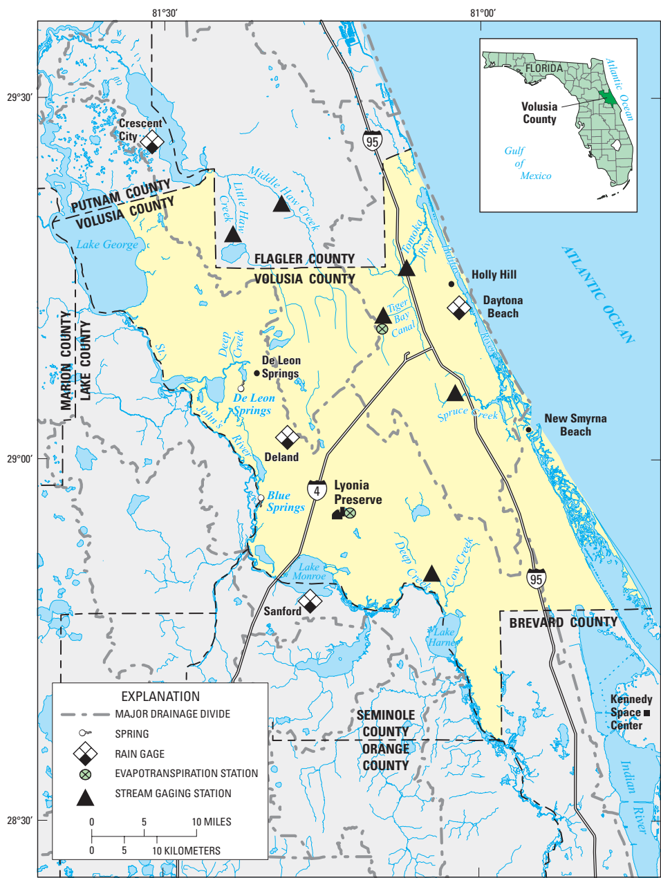
Figure 2. Surface drainage features and locations of hydrologic data stations.
