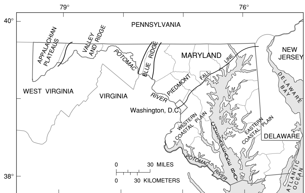
Figure 1. Study area and physiographic provinces in Maryland.
