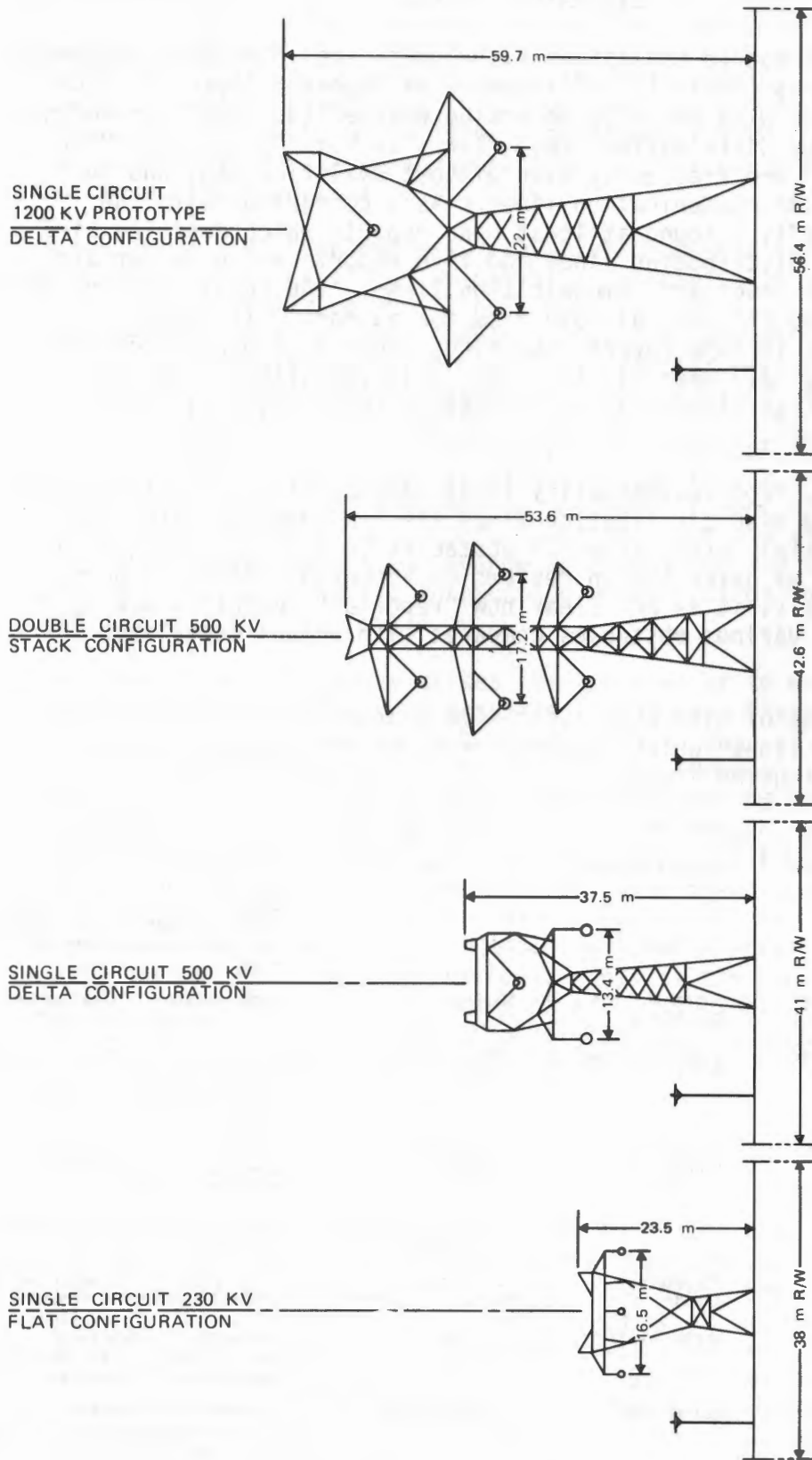
Figure 1. Configurations of typical BPA transmission towers. For comparison, a typical 125 kv distribution line pole, 10.4 m high, is shown to the left of each transmission tower.
