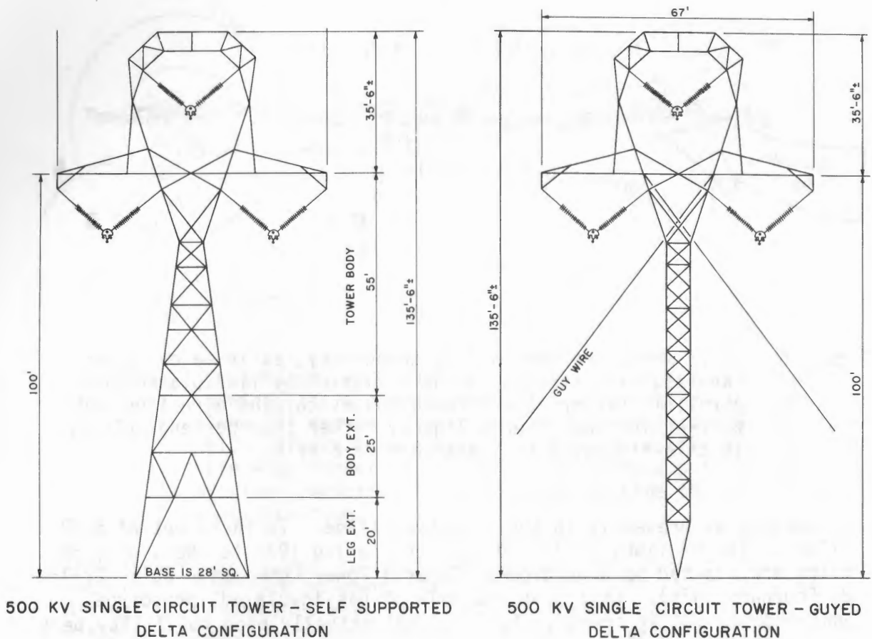
Figure 7. Self-supported and guyed 500 kV tower designs.
