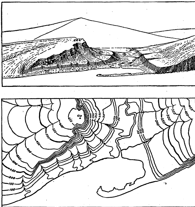
Fig. 1.—Ideal sketch and corresponding contour map.
