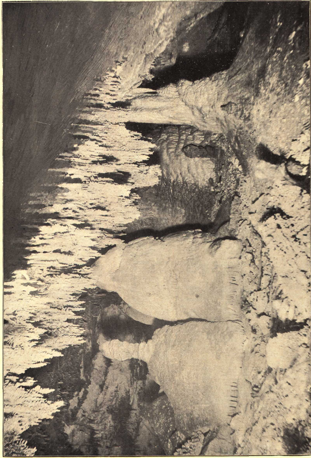
FIG. 3.—PORTION OF THE CAVE NEARLY FILLED WITH STALAGMITIC MATERIAL.
