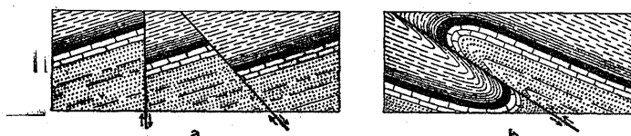
FIGURE 4.—Ideal sections of broken and bent strata, showing (a) normal faults and (b) a thrust or reverse fault.
