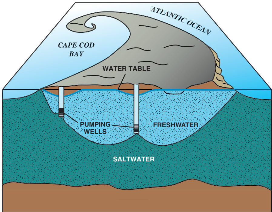
Figure 11. Overpumping from large-capacity municipal wells, such as those in the Pamet flow lens, can result in lateral encroachment and upconing of saltwater (modified from Strahler, 1972).
