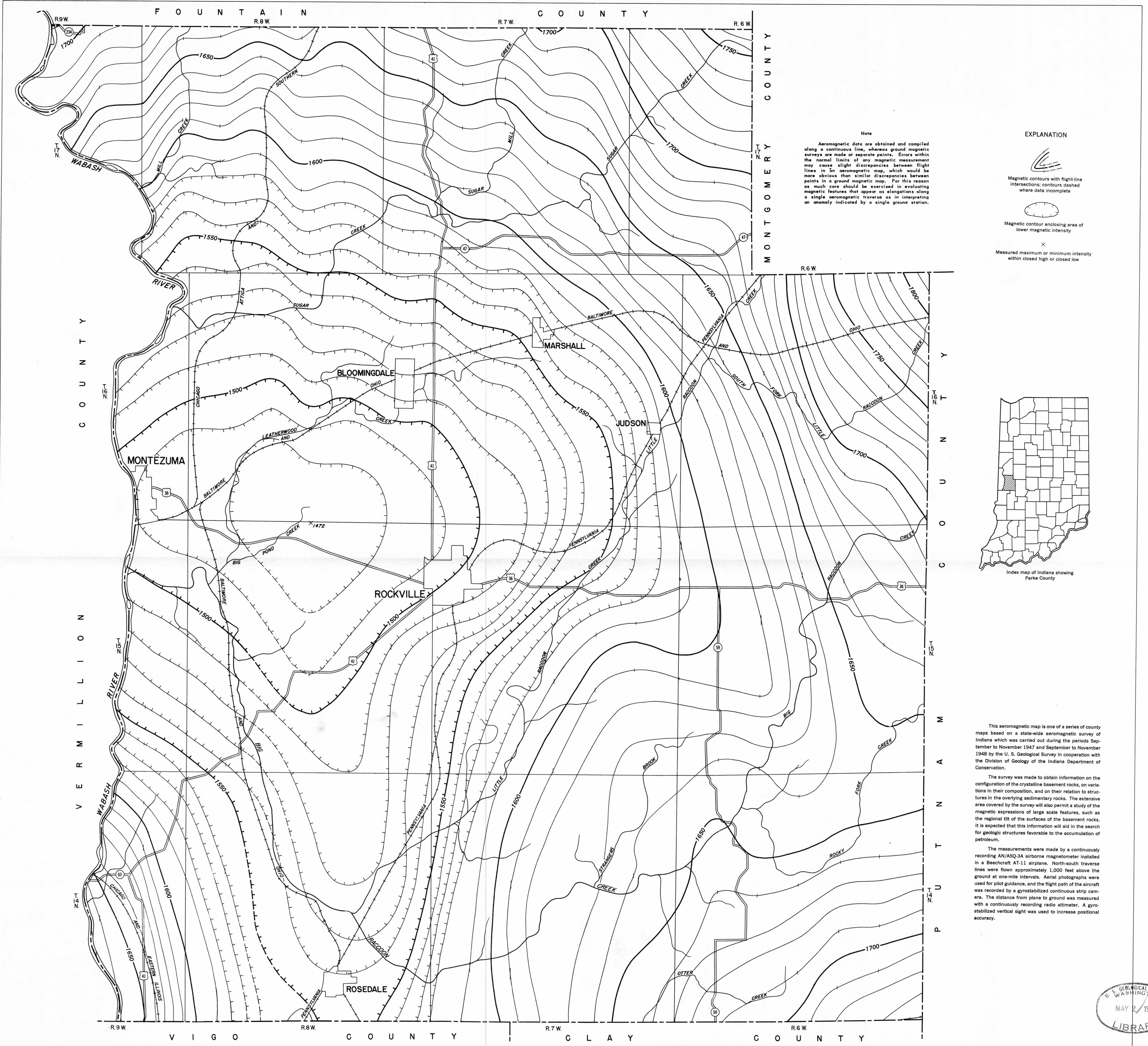
TOTAL INTENSITY AEROMAGNETIC MAP OF PARKE COUNTY, INDIANA RELATIVE TO ARBITRARY DATUM
