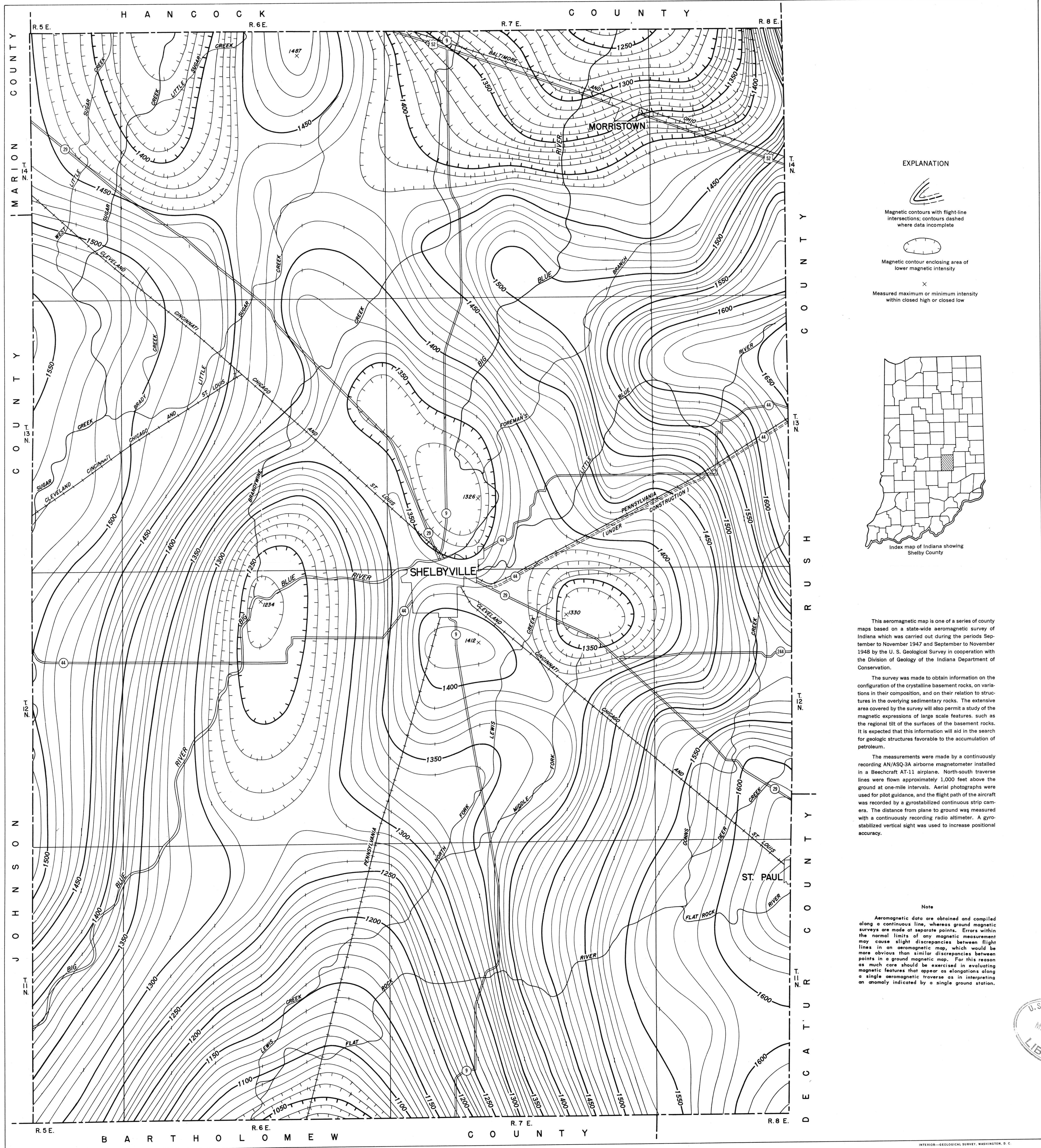
TOTAL INTENSITY AEROMAGNETIC MAP OF SHELBY COUNTY, INDIANA RELATIVE TO ARBITRARY DATUM
