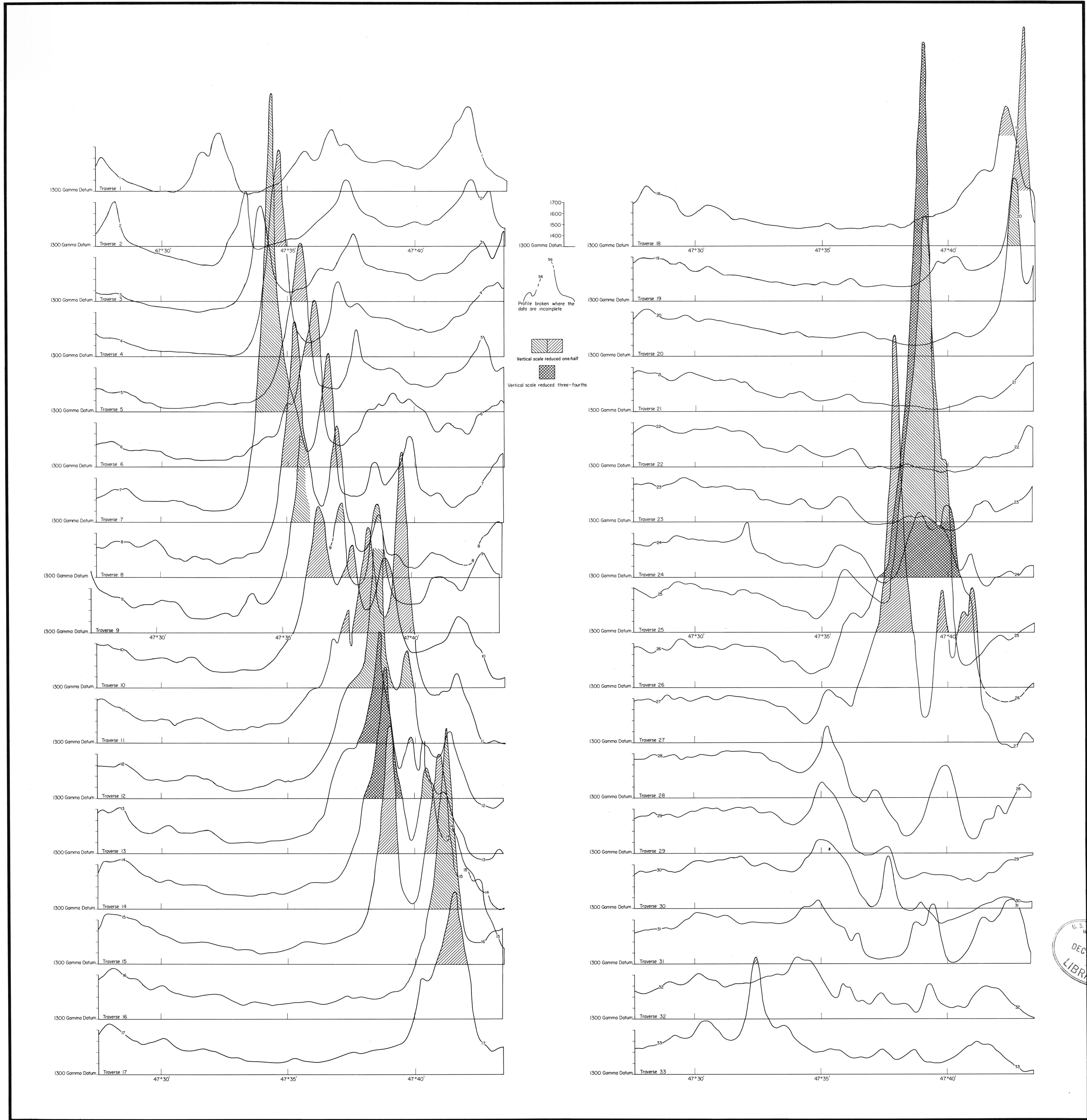
TOTAL INTENSITY AEROMAGNETIC PROFILES OF EAST-CENTRAL ITASCA COUNTY, MINNESOTA, TRAVERSES 1-33 RELATIVE TO ARBITRARY DATUM
