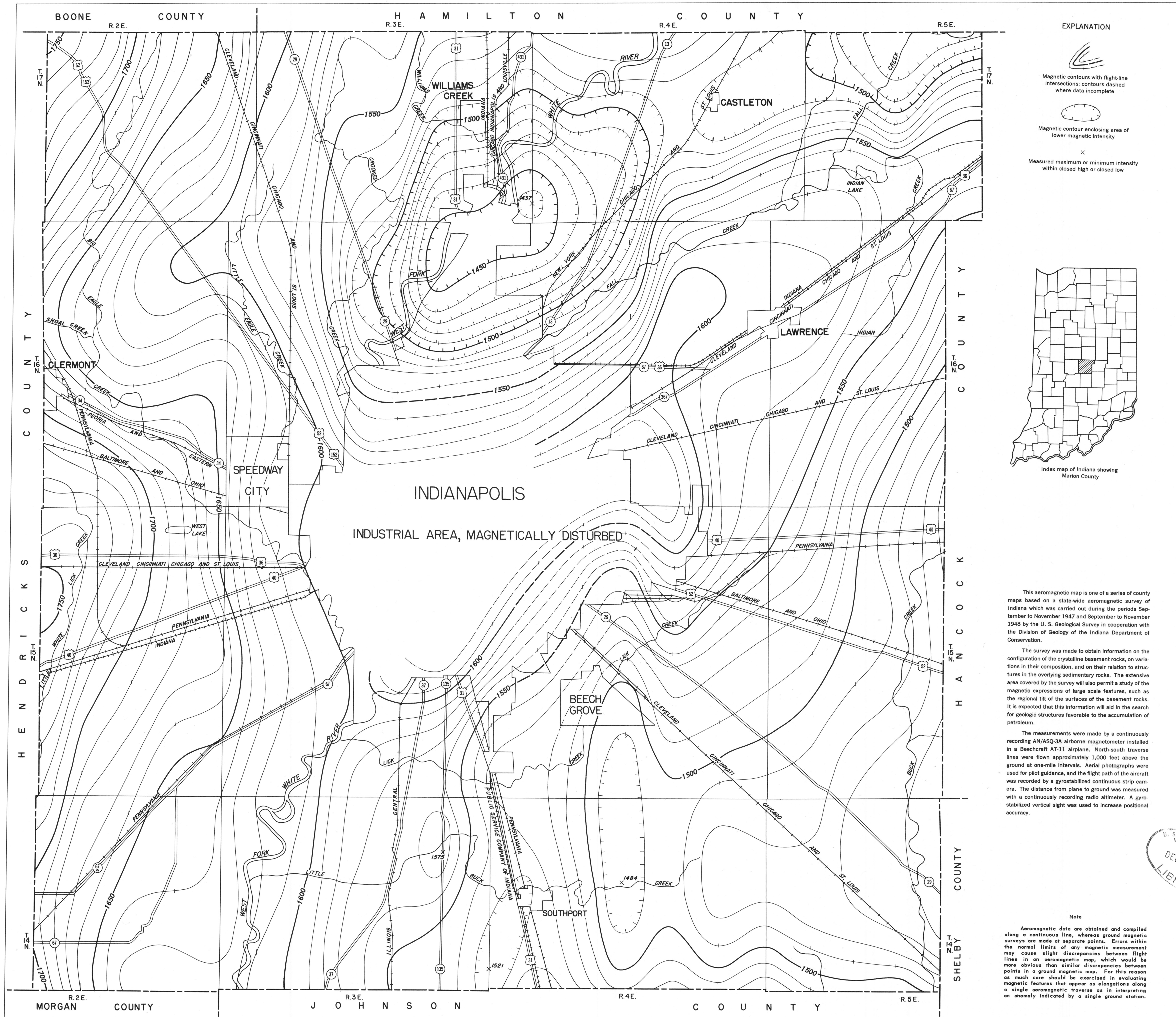
TOTAL INTENSITY AEROMAGNETIC MAP OF MARION COUNTY, INDIANA RELATIVE TO ARBITRARY DATUM
