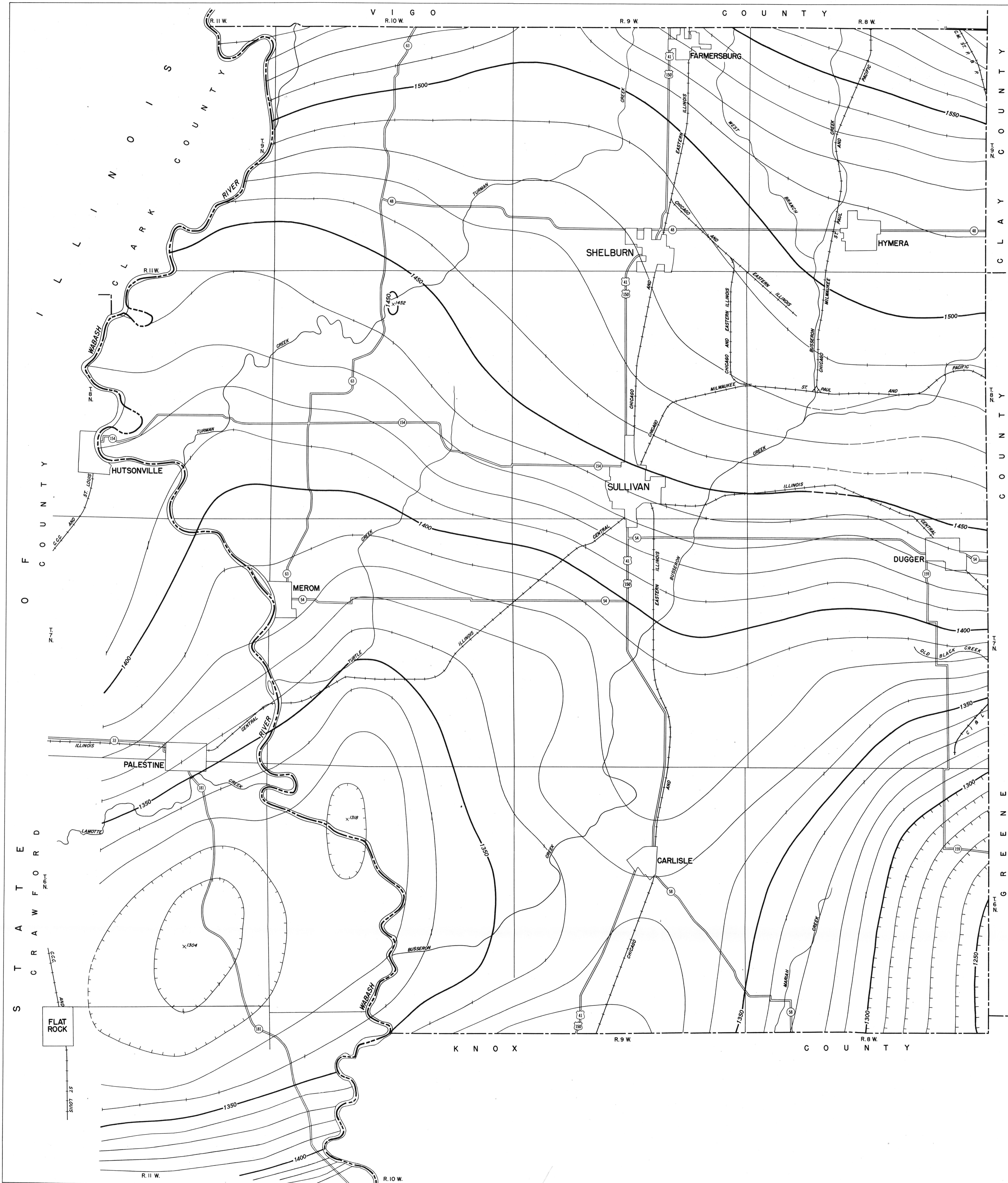
TOTAL INTENSITY AEROMAGNETIC MAP OF SULLIVAN COUNTY, INDIANA AND PART OF CRAWFORD COUNTY, ILLINOIS RELATIVE TO ARBITRARY DATUM
