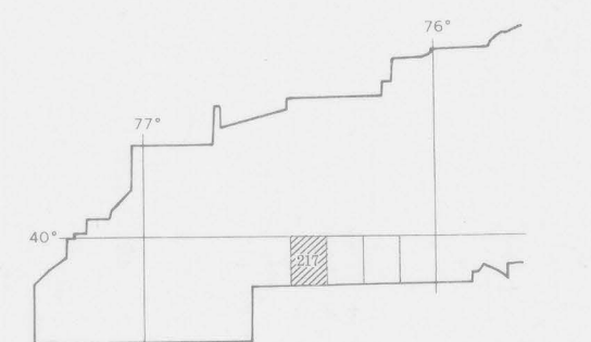
WESTERN PART OF AEROMAGNETIC SURVEY AREA SHOWING LOCATION OF THIS REPORT
